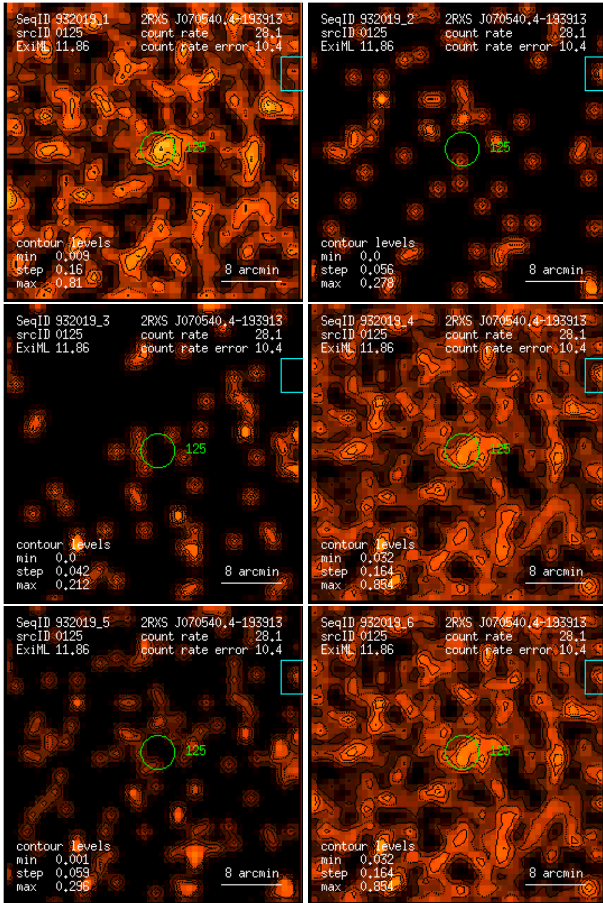
Figure 125: RASS 932019: detection 0125: band rate images, Gaussian filter: (1) PSPC channels 11 – 41, (2) 52 – 90, (3) 91 – 201, (4) 11 – 235, (5) 52 – 201, (6) 11 – 201. Broad band rates in counts/ks. Band rate contour levels in counts/ks/arcmin 2 .
