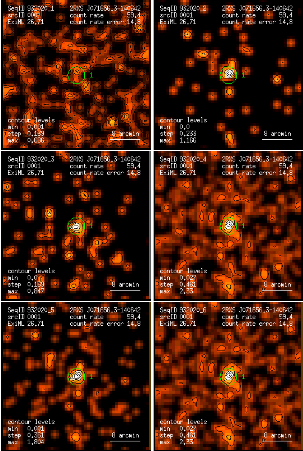
Figure 1: RASS 932020: detection 0001: band rate images, Gaussian filter: (1) PSPC channels 11 – 41, (2) 52 – 90, (3) 91 – 201, (4) 11 – 235, (5) 52 – 201, (6) 11 – 201. Broad band rates in counts/ks. Band rate contour levels in counts/ks/arcmin 2 .
