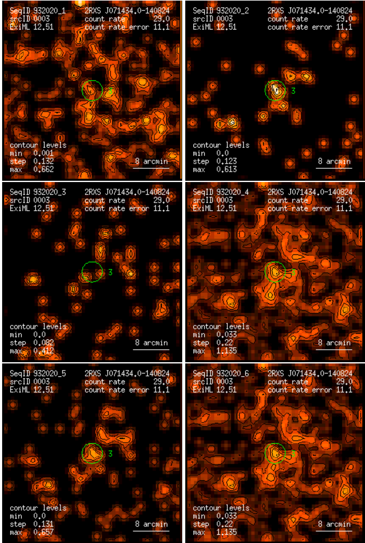
Figure 3: RASS 932020: detection 0003: band rate images, Gaussian filter: (1) PSPC channels 11 – 41, (2) 52 – 90, (3) 91 – 201, (4) 11 – 235, (5) 52 – 201, (6) 11 – 201. Broad band rates in counts/ks. Band rate contour levels in counts/ks/arcmin 2 .
