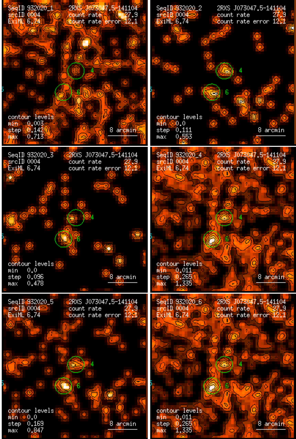
Figure 4: RASS 932020: detection 0004: band rate images, Gaussian filter: (1) PSPC channels 11 – 41, (2) 52 – 90, (3) 91 – 201, (4) 11 – 235, (5) 52 – 201, (6) 11 – 201. Broad band rates in counts/ks. Band rate contour levels in counts/ks/arcmin 2 .
