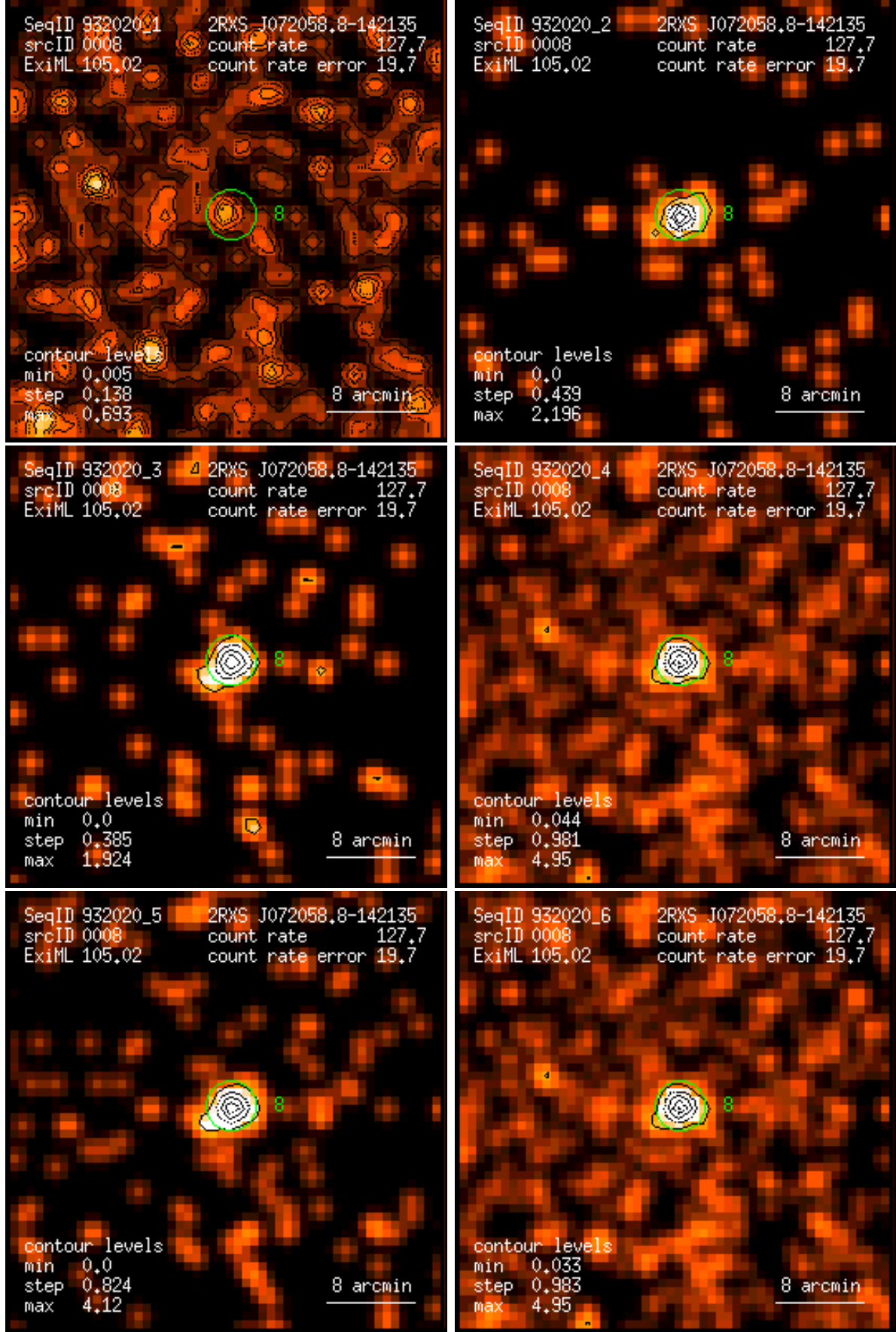
Figure 8: RASS 932020: detection 0008: band rate images, Gaussian filter: (1) PSPC channels 11 – 41, (2) 52 – 90, (3) 91 – 201, (4) 11 – 235, (5) 52 – 201, (6) 11 – 201. Broad band rates in counts/ks. Band rate contour levels in counts/ks/arcmin 2 .
