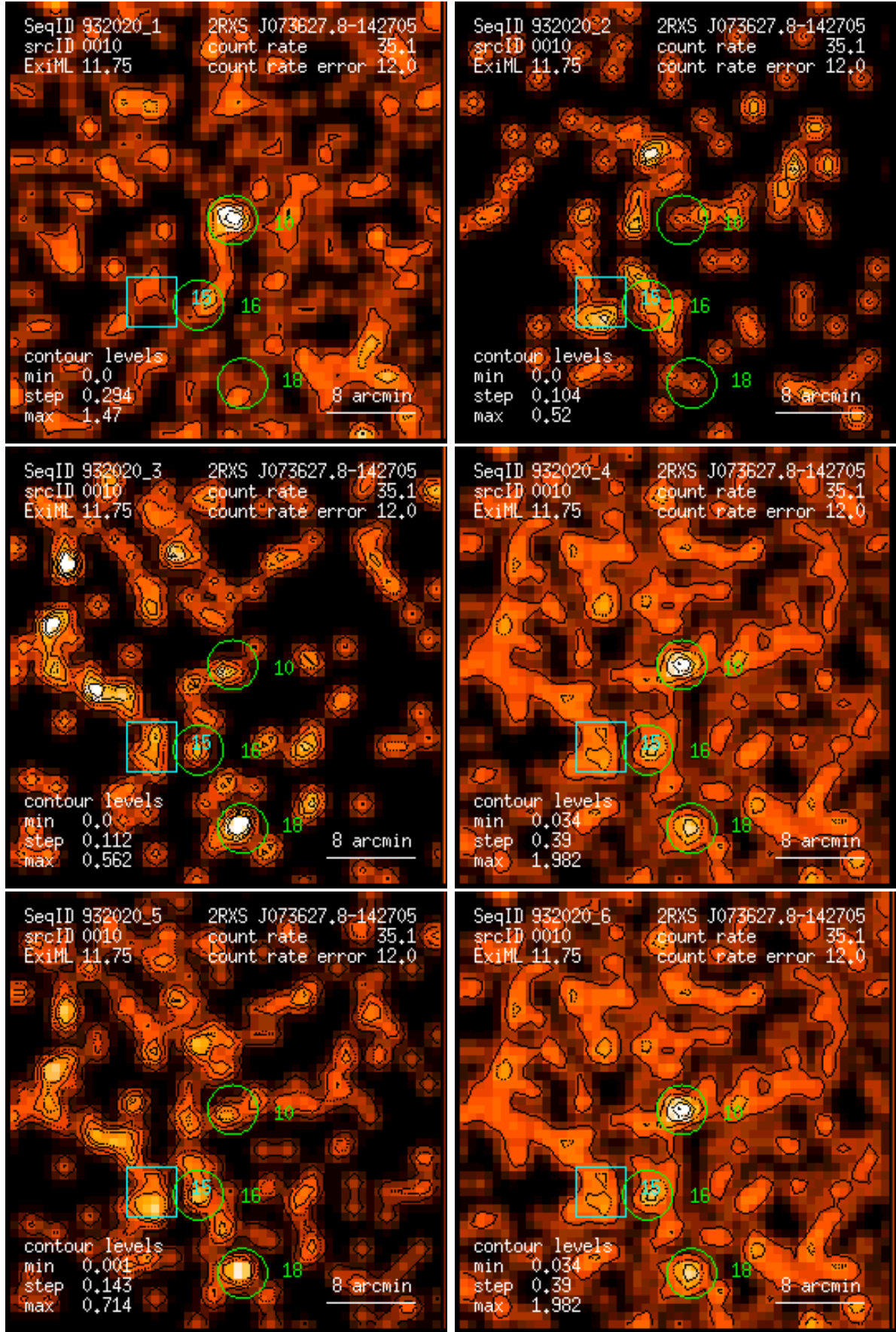
Figure 10: RASS 932020: detection 0010: band rate images, Gaussian filter: (1) PSPC channels 11 – 41, (2) 52 – 90, (3) 91 – 201, (4) 11 – 235, (5) 52 – 201, (6) 11 – 201. Broad band rates in counts/ks. Band rate contour levels in counts/ks/arcmin 2 .
