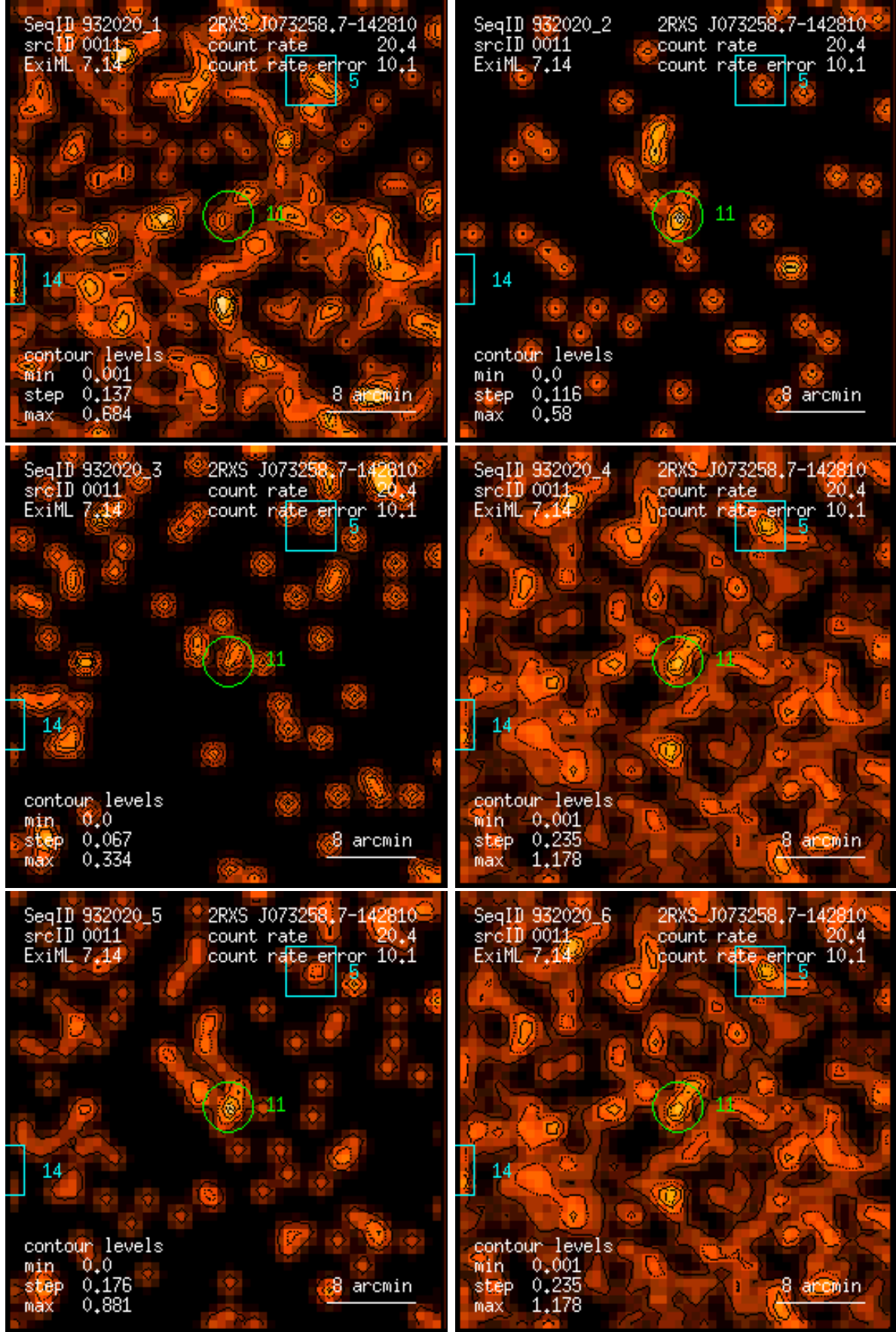
Figure 11: RASS 932020: detection 0011: band rate images, Gaussian filter: (1) PSPC channels 11 – 41, (2) 52 – 90, (3) 91 – 201, (4) 11 – 235, (5) 52 – 201, (6) 11 – 201. Broad band rates in counts/ks. Band rate contour levels in counts/ks/arcmin 2 .
