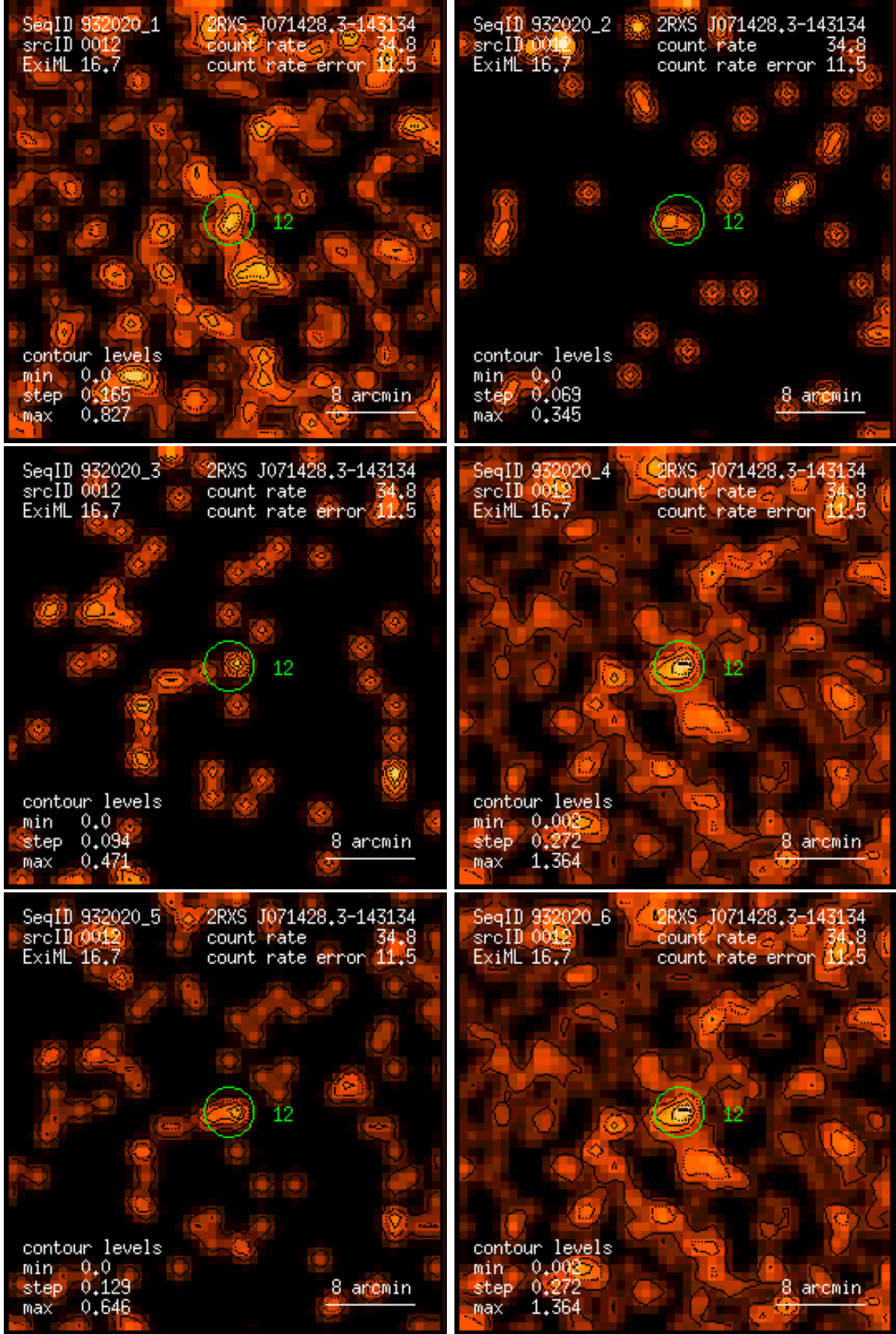
Figure 12: RASS 932020: detection 0012: band rate images, Gaussian filter: (1) PSPC channels 11 – 41, (2) 52 – 90, (3) 91 – 201, (4) 11 – 235, (5) 52 – 201, (6) 11 – 201. Broad band rates in counts/ks. Band rate contour levels in counts/ks/arcmin 2 .
