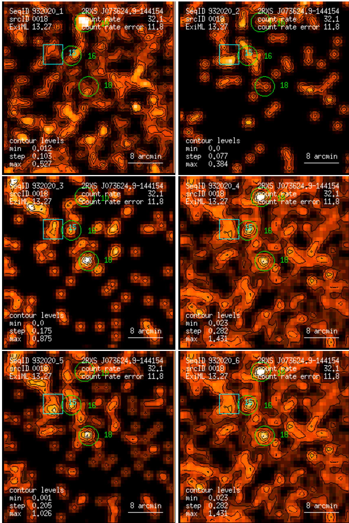
Figure 18: RASS 932020: detection 0018: band rate images, Gaussian filter: (1) PSPC channels 11 – 41, (2) 52 – 90, (3) 91 – 201, (4) 11 – 235, (5) 52 – 201, (6) 11 – 201. Broad band rates in counts/ks. Band rate contour levels in counts/ks/arcmin 2 .
