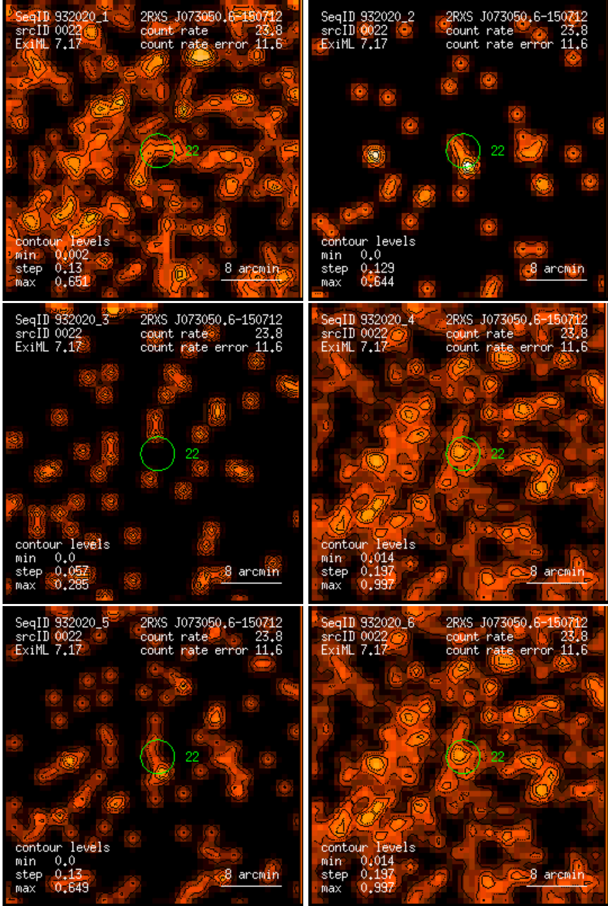
Figure 22: RASS 932020: detection 0022: band rate images, Gaussian filter: (1) PSPC channels 11 – 41, (2) 52 – 90, (3) 91 – 201, (4) 11 – 235, (5) 52 – 201, (6) 11 – 201. Broad band rates in counts/ks. Band rate contour levels in counts/ks/arcmin 2 .
