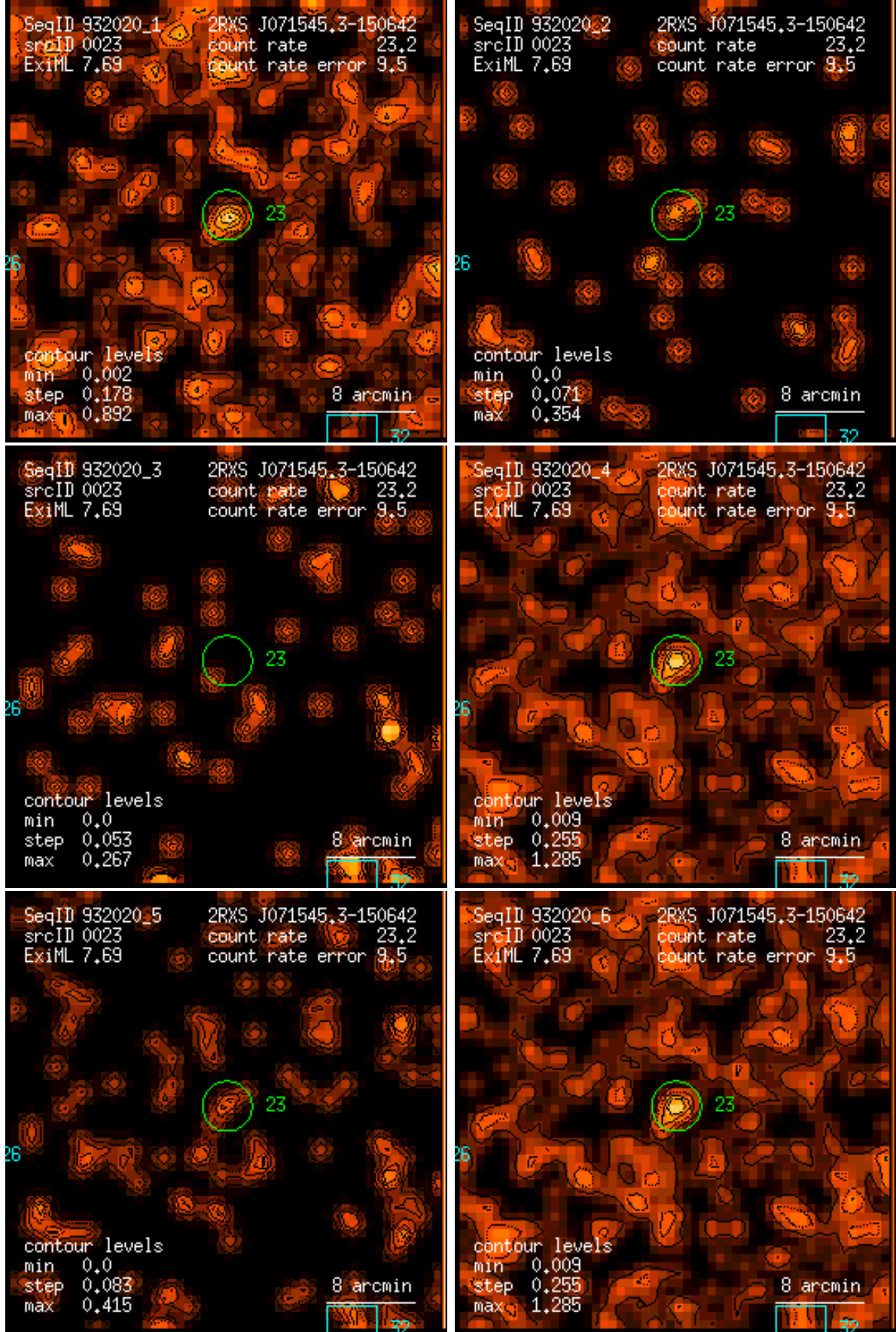
Figure 23: RASS 932020: detection 0023: band rate images, Gaussian filter: (1) PSPC channels 11 – 41, (2) 52 – 90, (3) 91 – 201, (4) 11 – 235, (5) 52 – 201, (6) 11 – 201. Broad band rates in counts/ks. Band rate contour levels in counts/ks/arcmin 2 .
