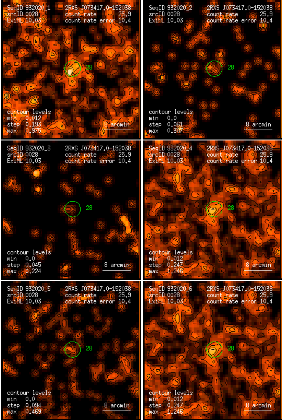
Figure 28: RASS 932020: detection 0028: band rate images, Gaussian filter: (1) PSPC channels 11 – 41, (2) 52 – 90, (3) 91 – 201, (4) 11 – 235, (5) 52 – 201, (6) 11 – 201. Broad band rates in counts/ks. Band rate contour levels in counts/ks/arcmin 2 .
