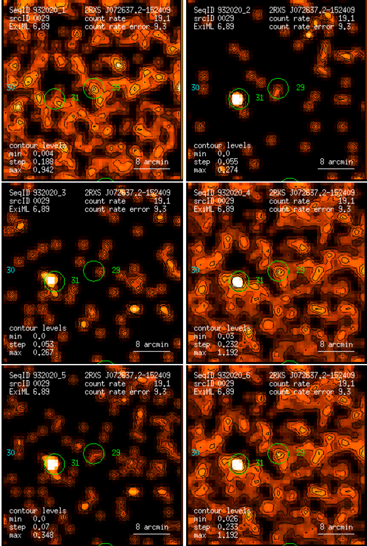
Figure 29: RASS 932020: detection 0029: band rate images, Gaussian filter: (1) PSPC channels 11 – 41, (2) 52 – 90, (3) 91 – 201, (4) 11 – 235, (5) 52 – 201, (6) 11 – 201. Broad band rates in counts/ks. Band rate contour levels in counts/ks/arcmin 2 .
