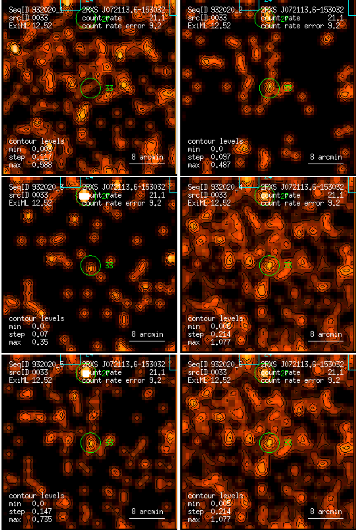
Figure 33: RASS 932020: detection 0033: band rate images, Gaussian filter: (1) PSPC channels 11 – 41, (2) 52 – 90, (3) 91 – 201, (4) 11 – 235, (5) 52 – 201, (6) 11 – 201. Broad band rates in counts/ks. Band rate contour levels in counts/ks/arcmin 2 .
