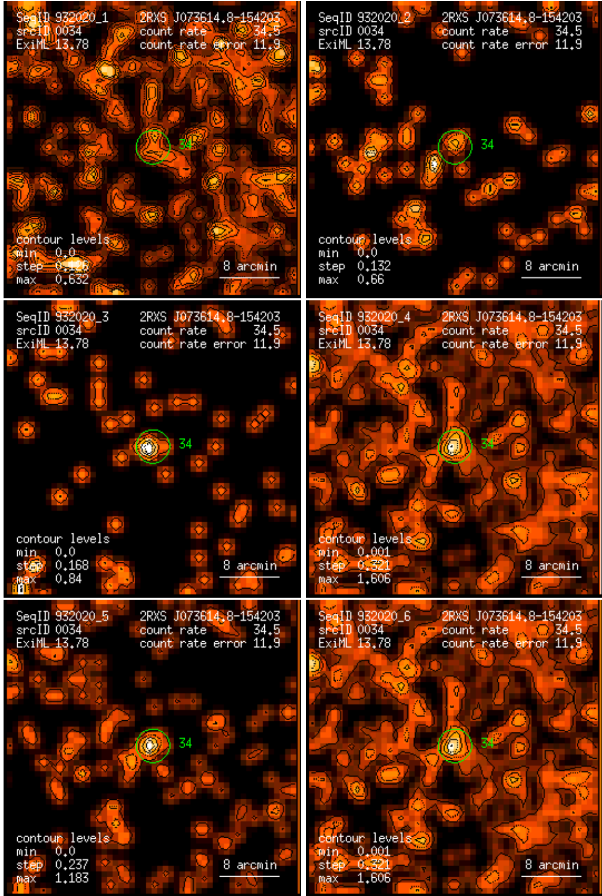
Figure 34: RASS 932020: detection 0034: band rate images, Gaussian filter: (1) PSPC channels 11 – 41, (2) 52 – 90, (3) 91 – 201, (4) 11 – 235, (5) 52 – 201, (6) 11 – 201. Broad band rates in counts/ks. Band rate contour levels in counts/ks/arcmin 2 .
