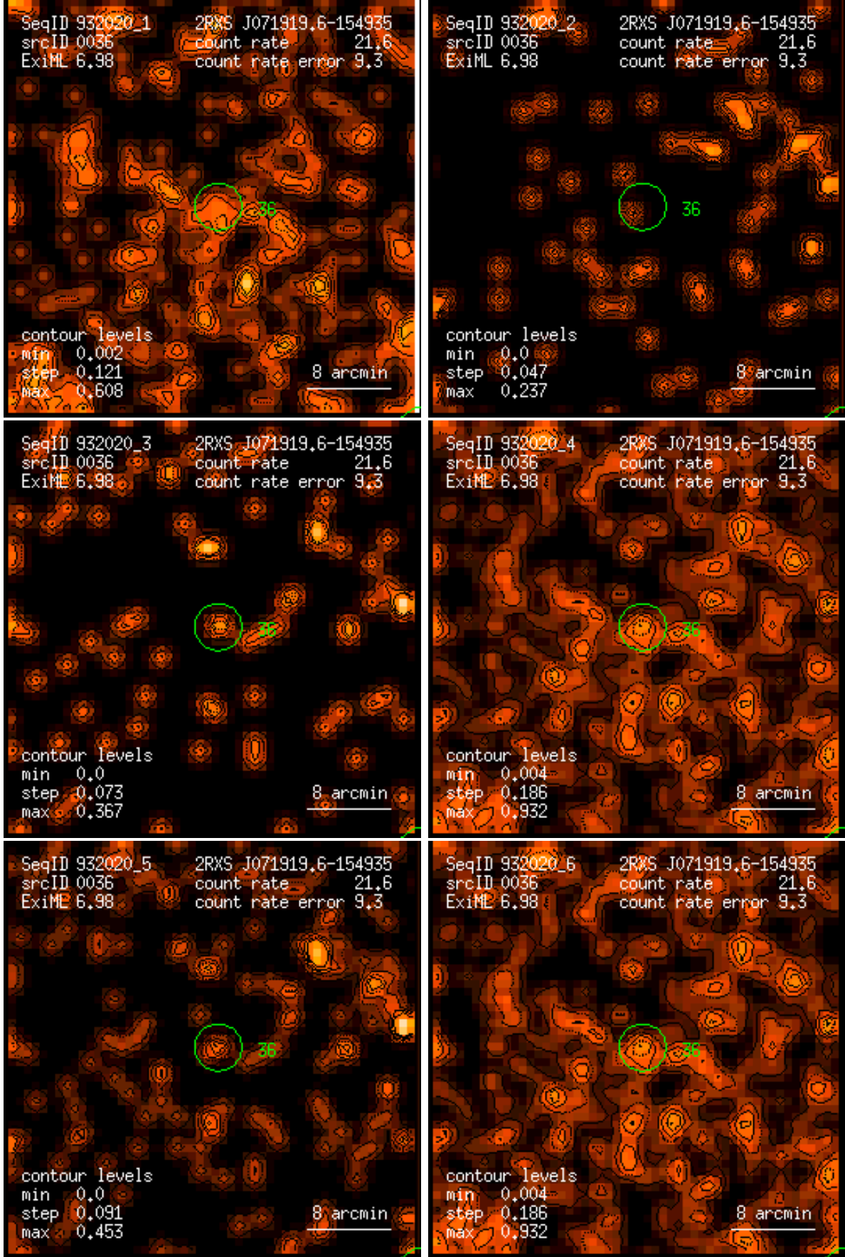
Figure 36: RASS 932020: detection 0036: band rate images, Gaussian filter: (1) PSPC channels 11 – 41, (2) 52 – 90, (3) 91 – 201, (4) 11 – 235, (5) 52 – 201, (6) 11 – 201. Broad band rates in counts/ks. Band rate contour levels in counts/ks/arcmin 2 .
