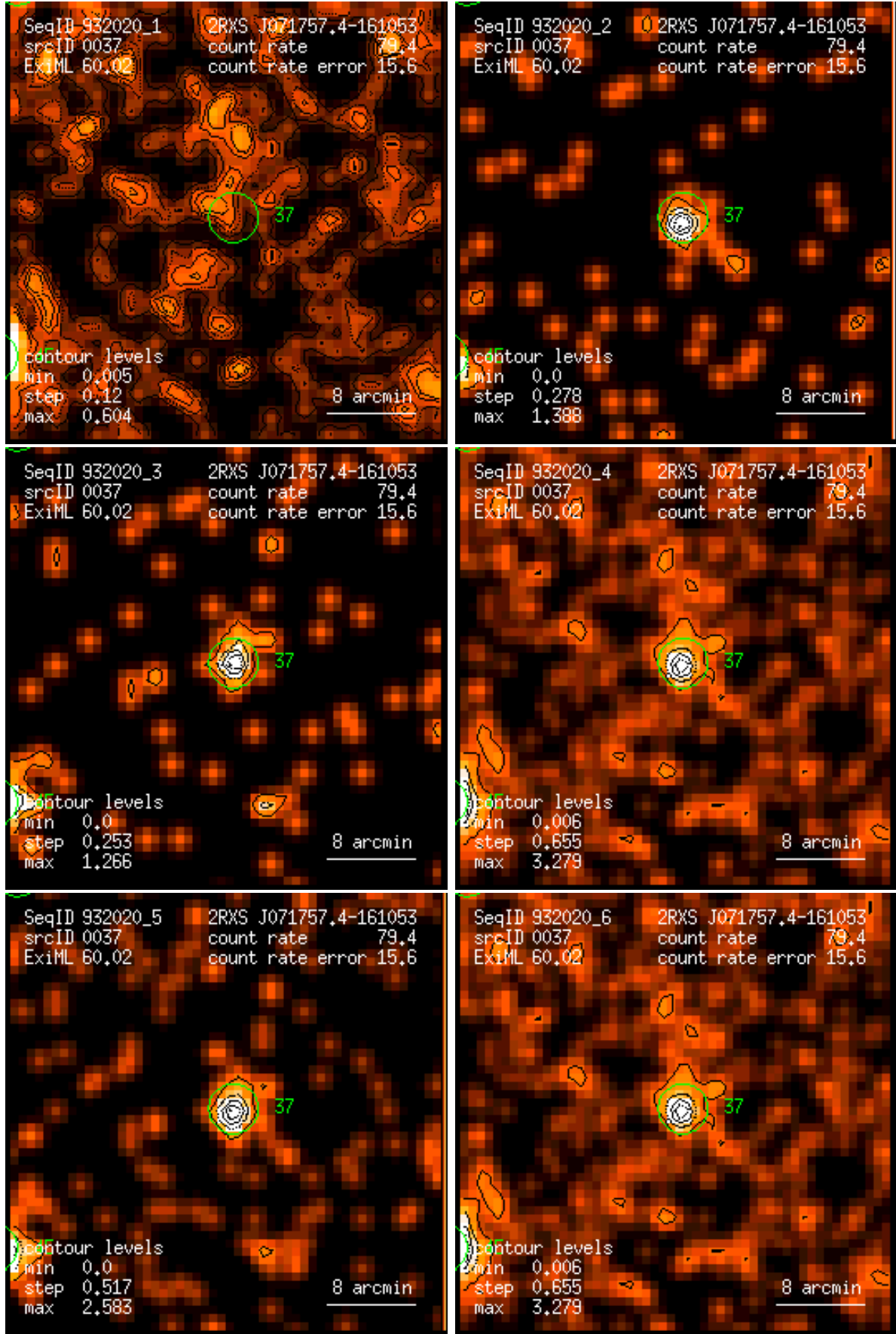
Figure 37: RASS 932020: detection 0037: band rate images, Gaussian filter: (1) PSPC channels 11 – 41, (2) 52 – 90, (3) 91 – 201, (4) 11 – 235, (5) 52 – 201, (6) 11 – 201. Broad band rates in counts/ks. Band rate contour levels in counts/ks/arcmin 2 .
