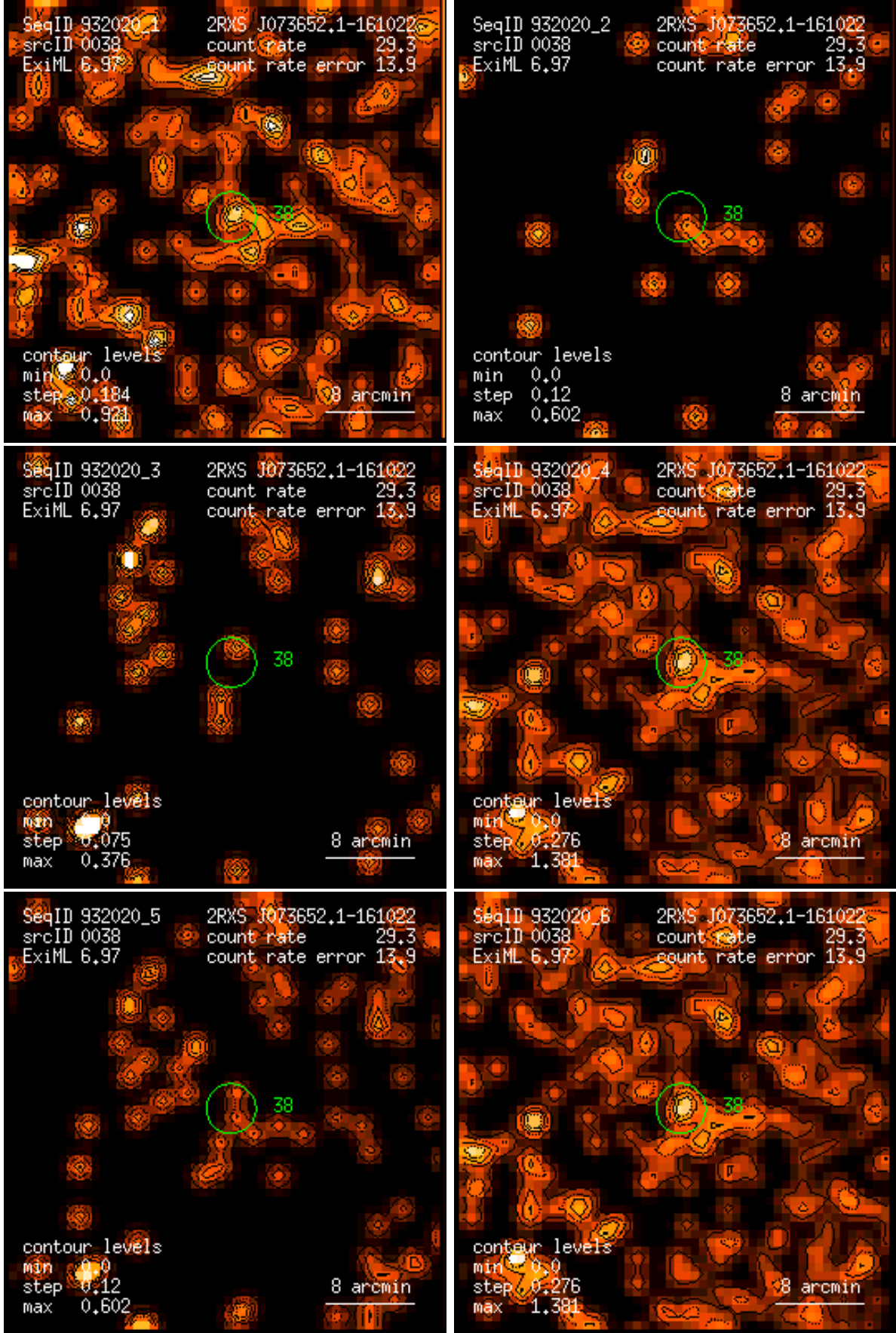
Figure 38: RASS 932020: detection 0038: band rate images, Gaussian filter: (1) PSPC channels 11 – 41, (2) 52 – 90, (3) 91 – 201, (4) 11 – 235, (5) 52 – 201, (6) 11 – 201. Broad band rates in counts/ks. Band rate contour levels in counts/ks/arcmin 2 .
