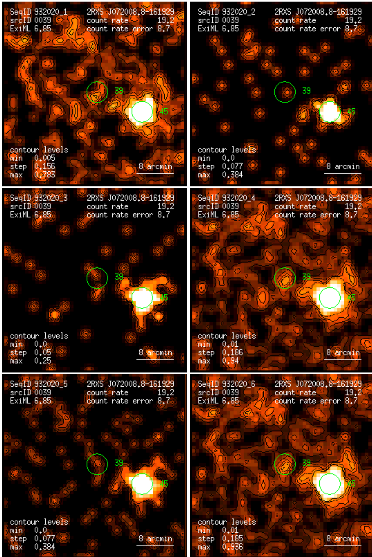
Figure 39: RASS 932020: detection 0039: band rate images, Gaussian filter: (1) PSPC channels 11 – 41, (2) 52 – 90, (3) 91 – 201, (4) 11 – 235, (5) 52 – 201, (6) 11 – 201. Broad band rates in counts/ks. Band rate contour levels in counts/ks/arcmin 2 .
