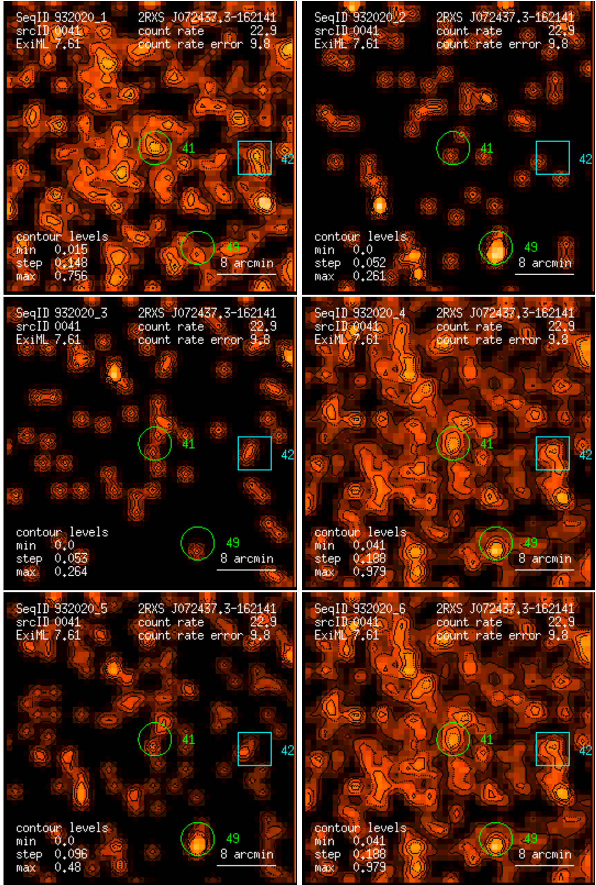
Figure 41: RASS 932020: detection 0041: band rate images, Gaussian filter: (1) PSPC channels 11 – 41, (2) 52 – 90, (3) 91 – 201, (4) 11 – 235, (5) 52 – 201, (6) 11 – 201. Broad band rates in counts/ks. Band rate contour levels in counts/ks/arcmin 2 .
