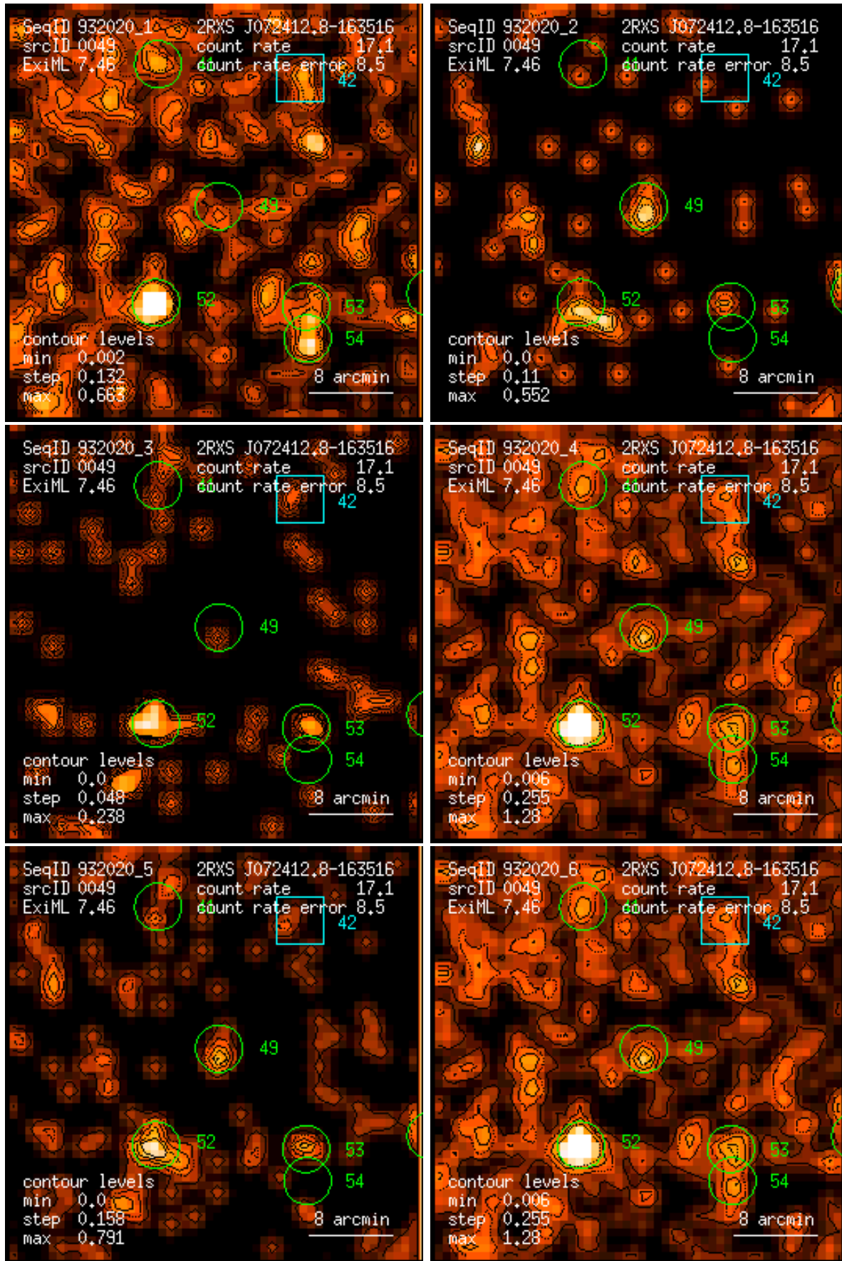
Figure 49: RASS 932020: detection 0049: band rate images, Gaussian filter: (1) PSPC channels 11 – 41, (2) 52 – 90, (3) 91 – 201, (4) 11 – 235, (5) 52 – 201, (6) 11 – 201. Broad band rates in counts/ks. Band rate contour levels in counts/ks/arcmin 2 .
