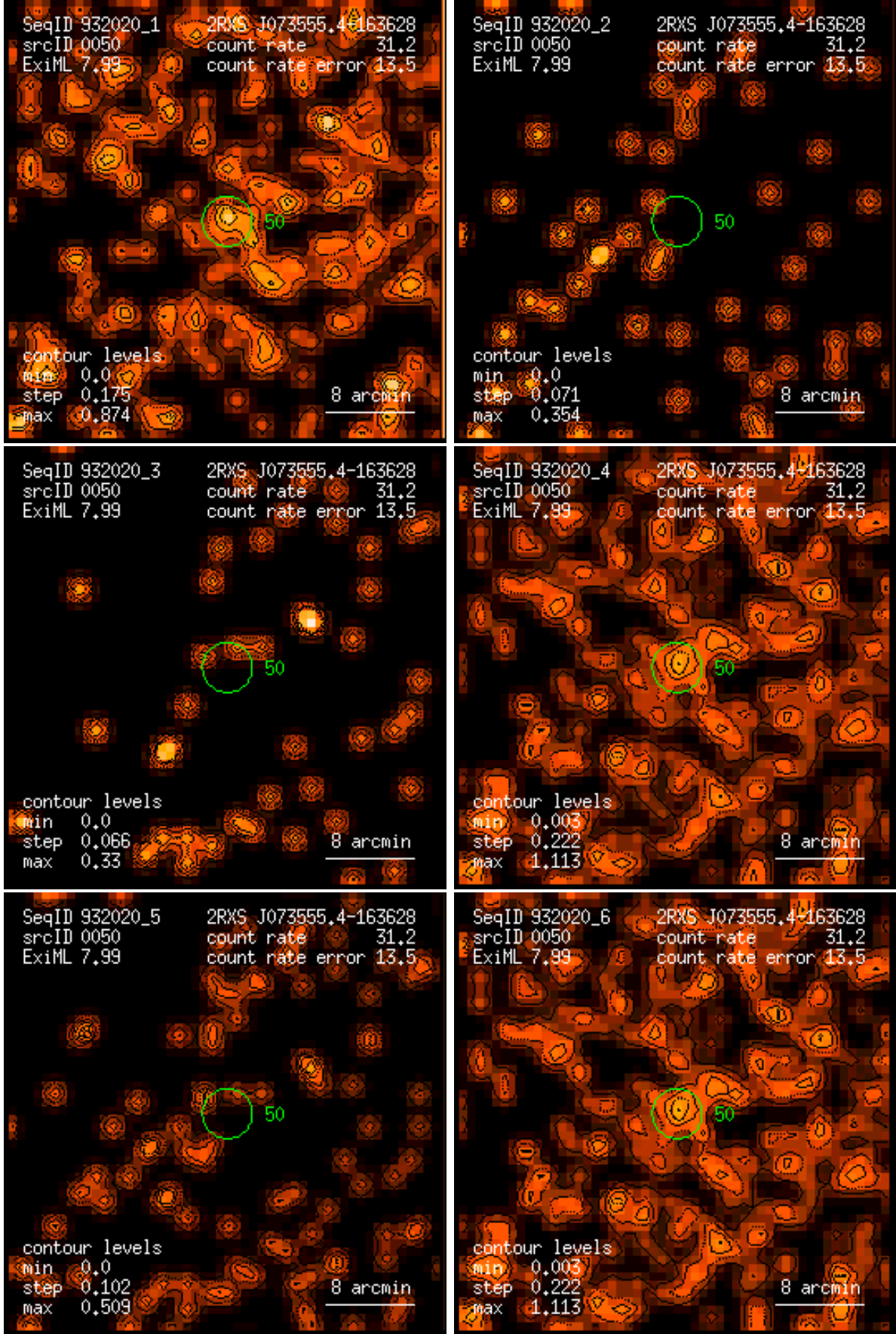
Figure 50: RASS 932020: detection 0050: band rate images, Gaussian filter: (1) PSPC channels 11 – 41, (2) 52 – 90, (3) 91 – 201, (4) 11 – 235, (5) 52 – 201, (6) 11 – 201. Broad band rates in counts/ks. Band rate contour levels in counts/ks/arcmin 2 .
