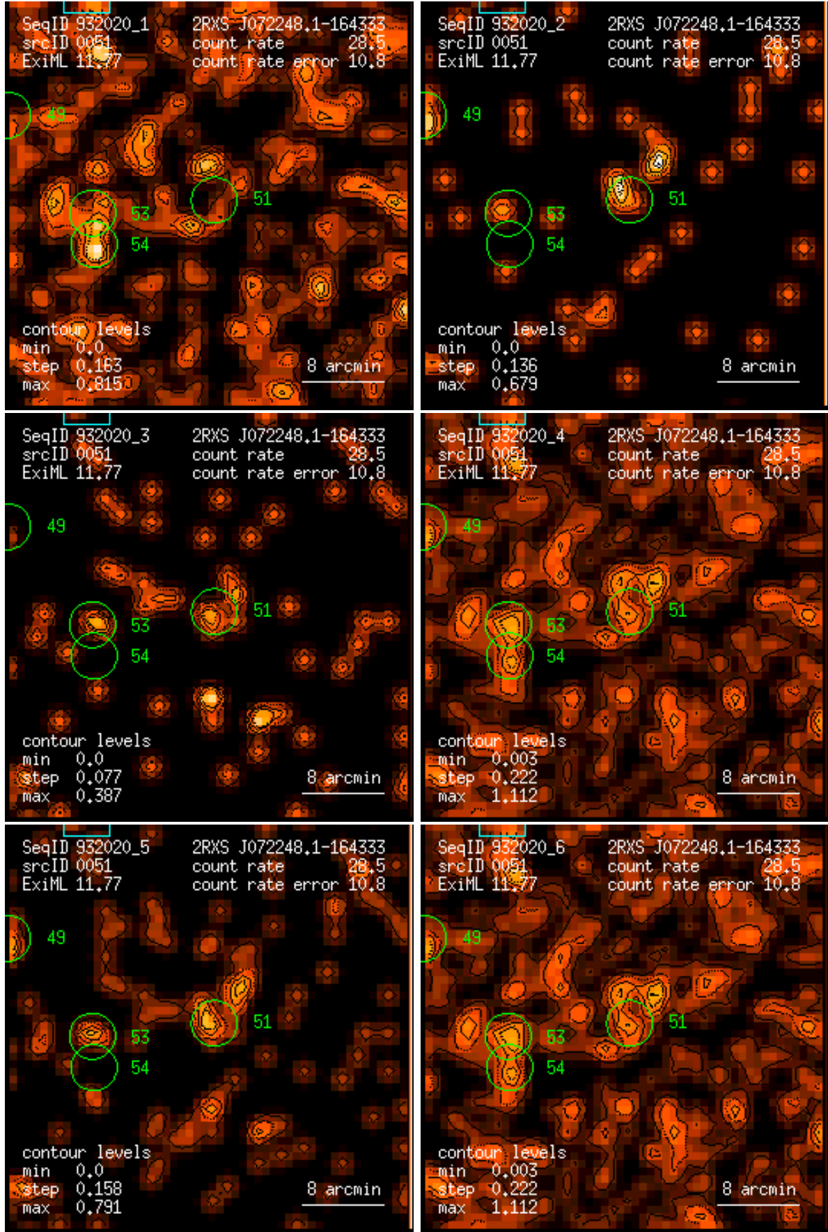
Figure 51: RASS 932020: detection 0051: band rate images, Gaussian filter: (1) PSPC channels 11 – 41, (2) 52 – 90, (3) 91 – 201, (4) 11 – 235, (5) 52 – 201, (6) 11 – 201. Broad band rates in counts/ks. Band rate contour levels in counts/ks/arcmin 2 .
