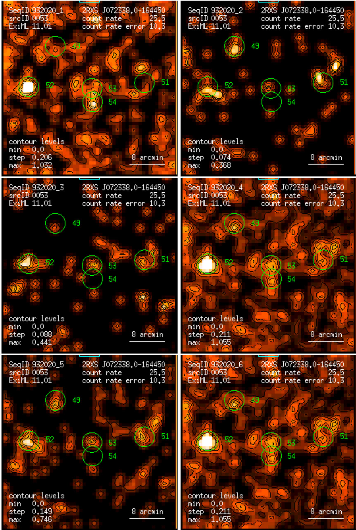
Figure 53: RASS 932020: detection 0053: band rate images, Gaussian filter: (1) PSPC channels 11 – 41, (2) 52 – 90, (3) 91 – 201, (4) 11 – 235, (5) 52 – 201, (6) 11 – 201. Broad band rates in counts/ks. Band rate contour levels in counts/ks/arcmin 2 .
