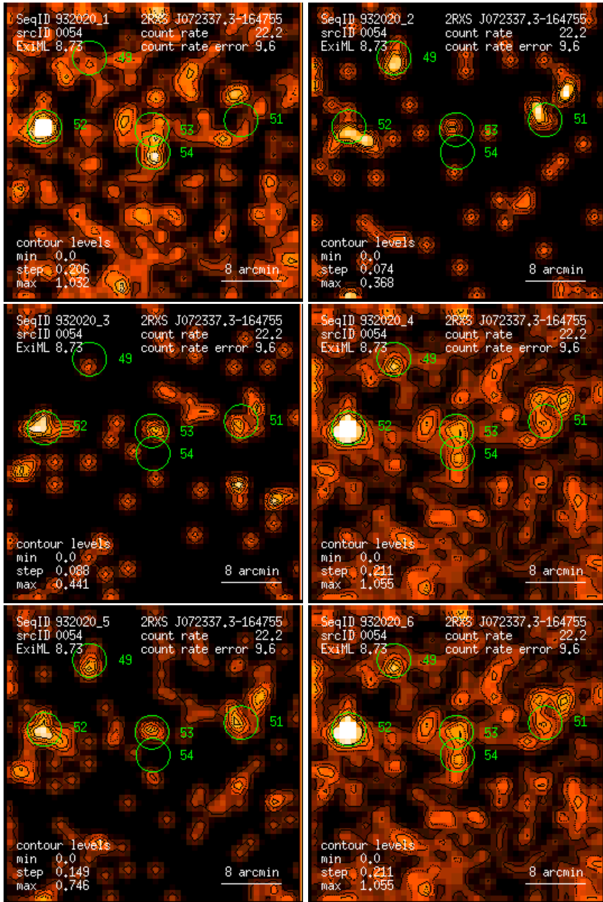
Figure 54: RASS 932020: detection 0054: band rate images, Gaussian filter: (1) PSPC channels 11 – 41, (2) 52 – 90, (3) 91 – 201, (4) 11 – 235, (5) 52 – 201, (6) 11 – 201. Broad band rates in counts/ks. Band rate contour levels in counts/ks/arcmin 2 .
