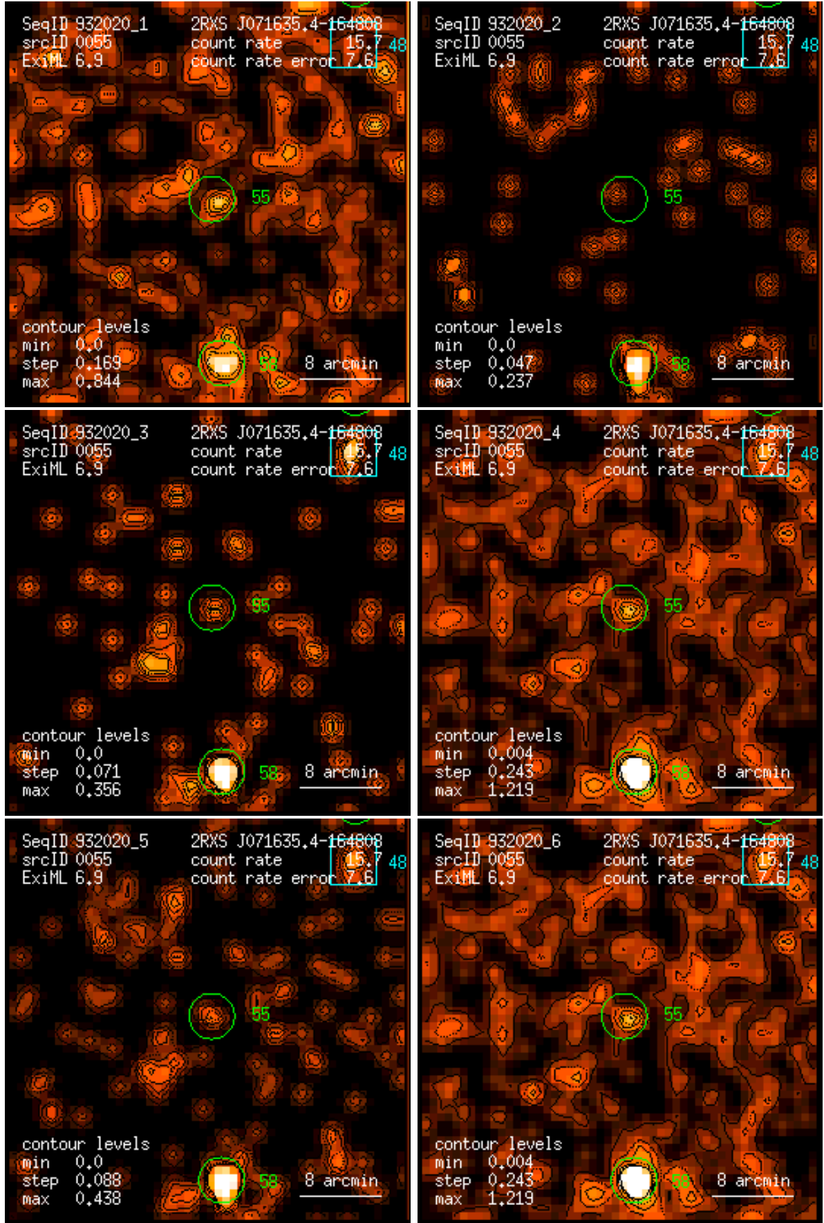
Figure 55: RASS 932020: detection 0055: band rate images, Gaussian filter: (1) PSPC channels 11 – 41, (2) 52 – 90, (3) 91 – 201, (4) 11 – 235, (5) 52 – 201, (6) 11 – 201. Broad band rates in counts/ks. Band rate contour levels in counts/ks/arcmin 2 .
