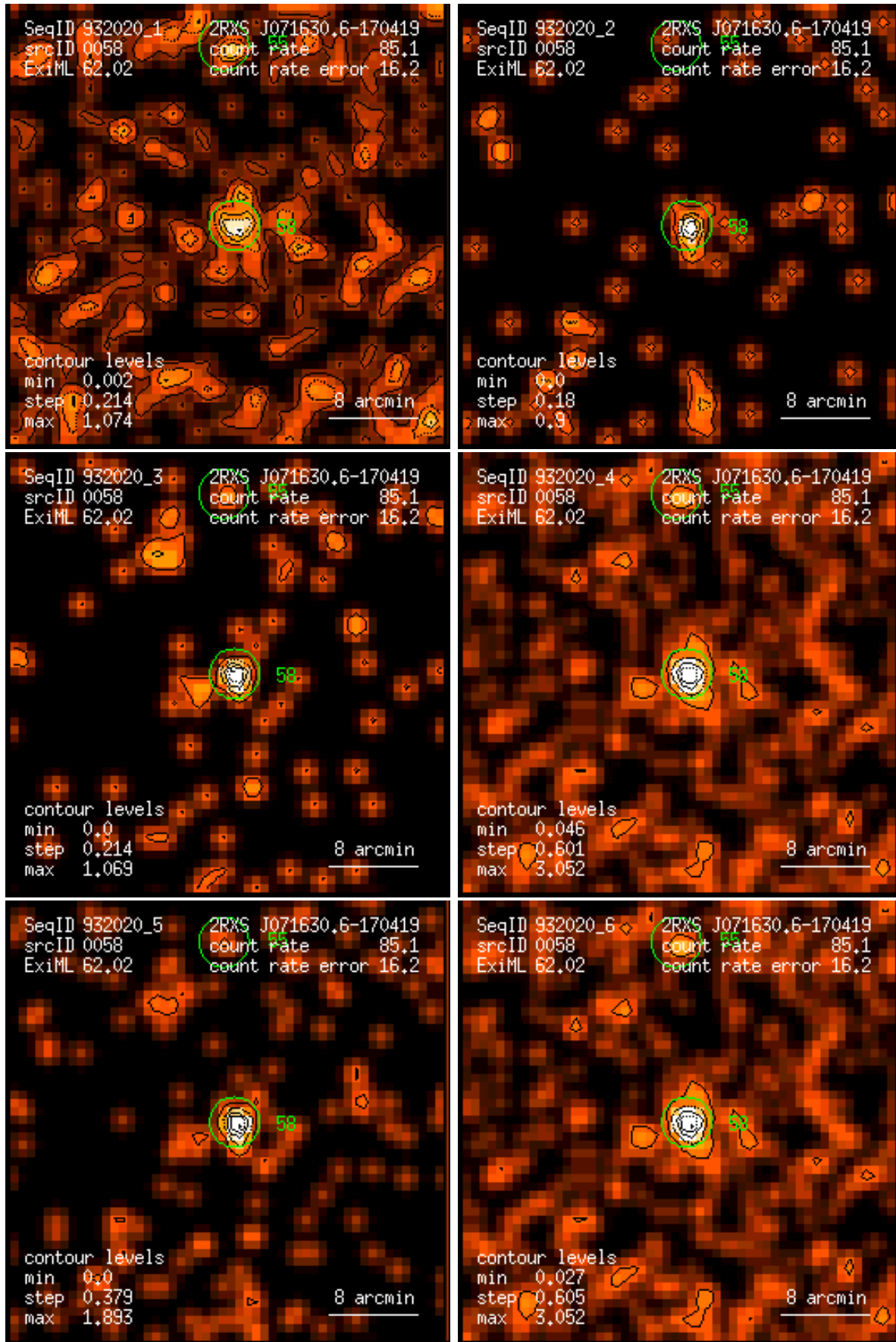
Figure 58: RASS 932020: detection 0058: band rate images, Gaussian filter: (1) PSPC channels 11 – 41, (2) 52 – 90, (3) 91 – 201, (4) 11 – 235, (5) 52 – 201, (6) 11 – 201. Broad band rates in counts/ks. Band rate contour levels in counts/ks/arcmin 2 .
