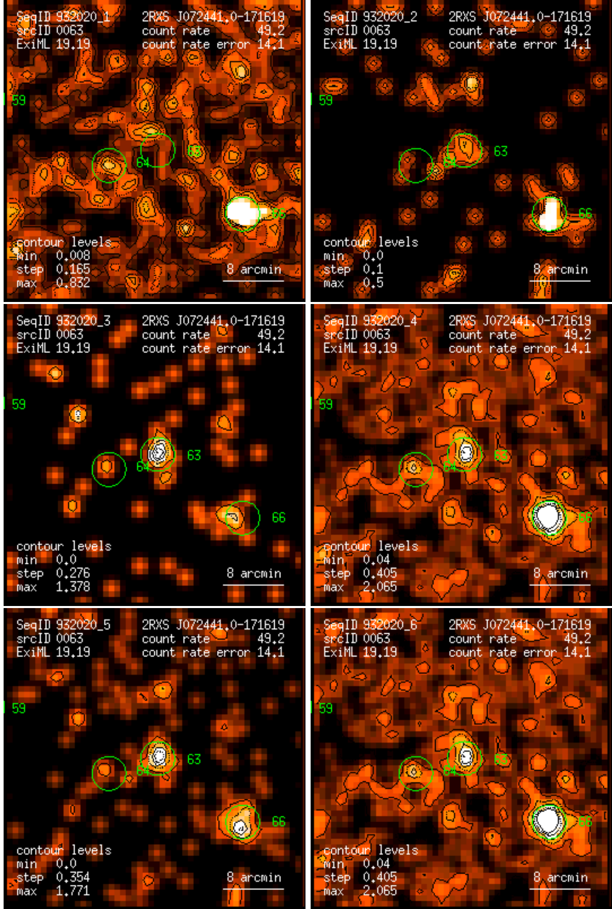
Figure 63: RASS 932020: detection 0063: band rate images, Gaussian filter: (1) PSPC channels 11 – 41, (2) 52 – 90, (3) 91 – 201, (4) 11 – 235, (5) 52 – 201, (6) 11 – 201. Broad band rates in counts/ks. Band rate contour levels in counts/ks/arcmin 2 .
