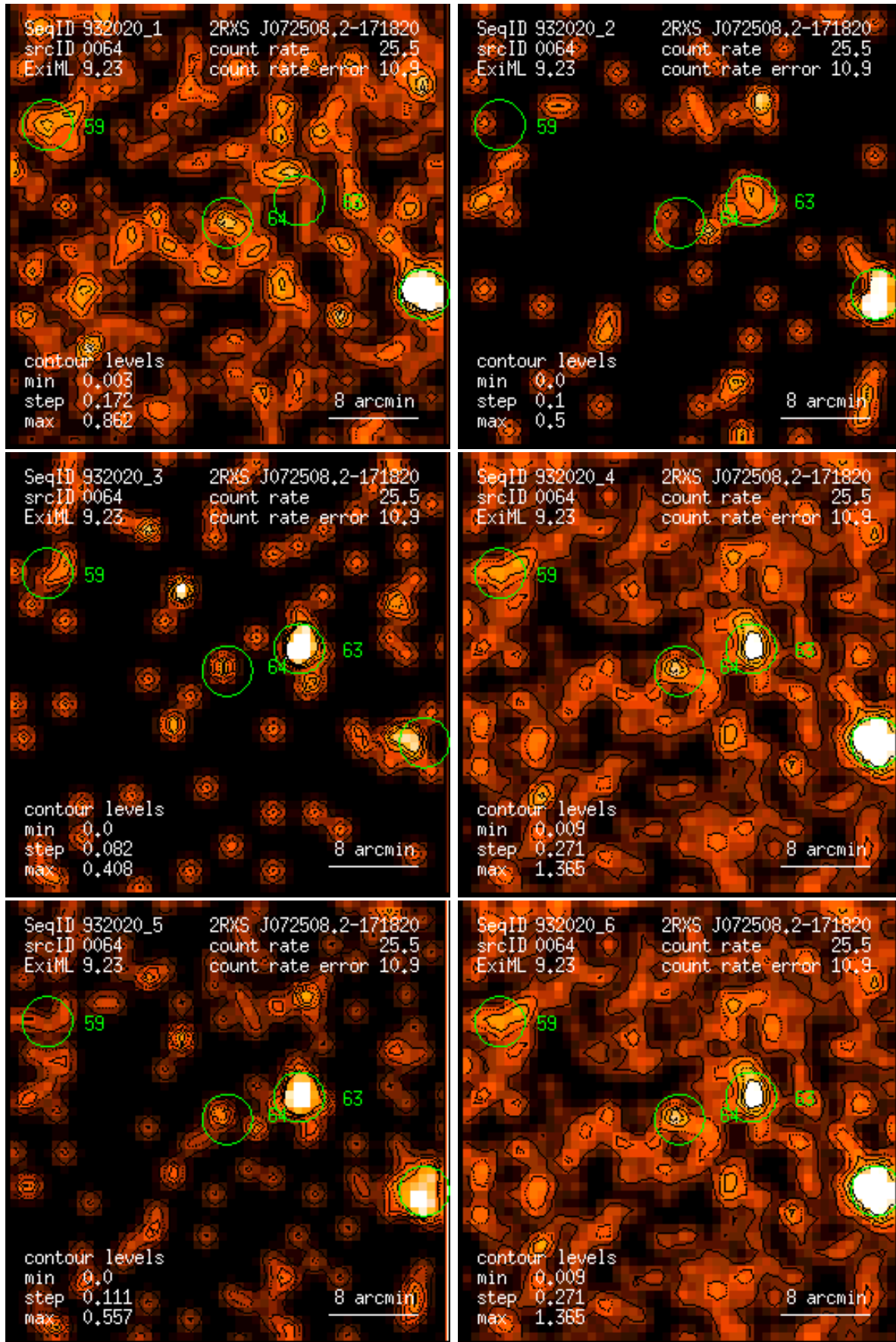
Figure 64: RASS 932020: detection 0064: band rate images, Gaussian filter: (1) PSPC channels 11 – 41, (2) 52 – 90, (3) 91 – 201, (4) 11 – 235, (5) 52 – 201, (6) 11 – 201. Broad band rates in counts/ks. Band rate contour levels in counts/ks/arcmin 2 .
