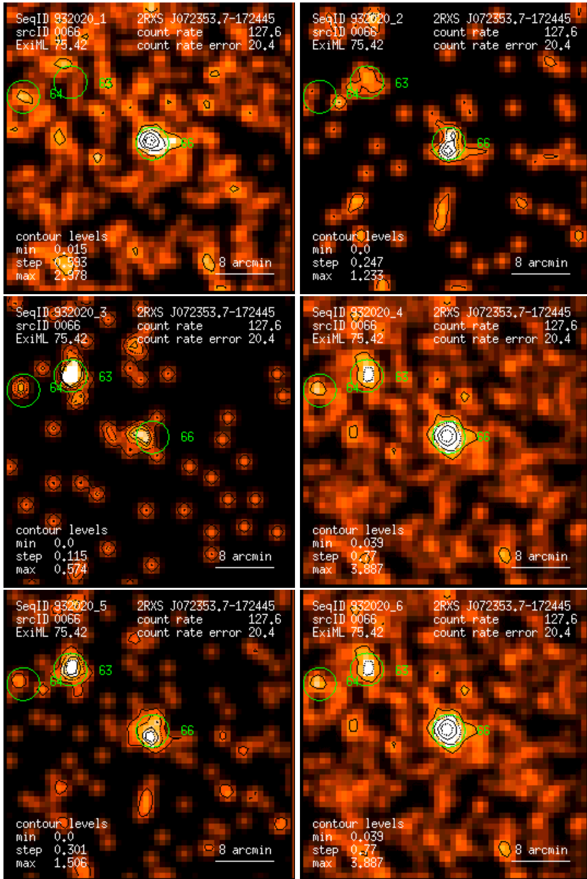
Figure 66: RASS 932020: detection 0066: band rate images, Gaussian filter: (1) PSPC channels 11 – 41, (2) 52 – 90, (3) 91 – 201, (4) 11 – 235, (5) 52 – 201, (6) 11 – 201. Broad band rates in counts/ks. Band rate contour levels in counts/ks/arcmin 2 .
