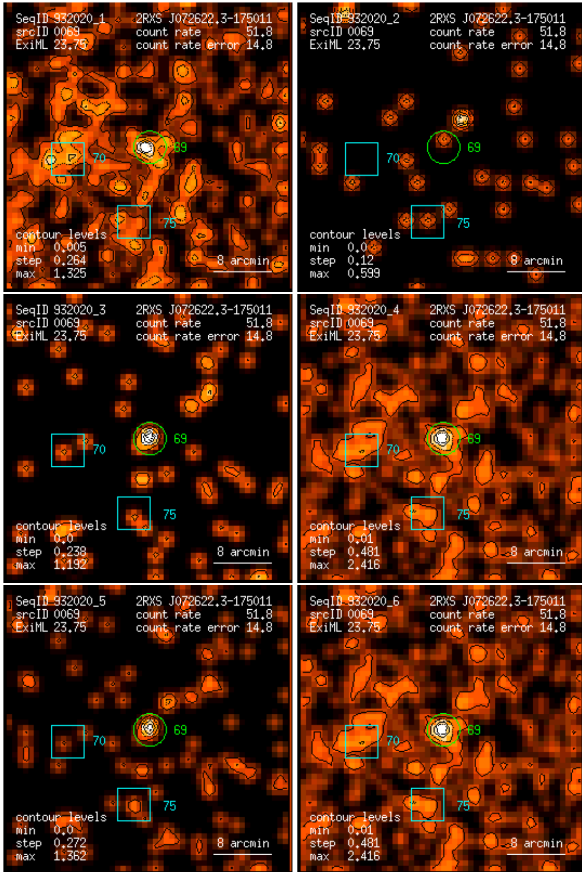
Figure 69: RASS 932020: detection 0069: band rate images, Gaussian filter: (1) PSPC channels 11 – 41, (2) 52 – 90, (3) 91 – 201, (4) 11 – 235, (5) 52 – 201, (6) 11 – 201. Broad band rates in counts/ks. Band rate contour levels in counts/ks/arcmin 2 .
