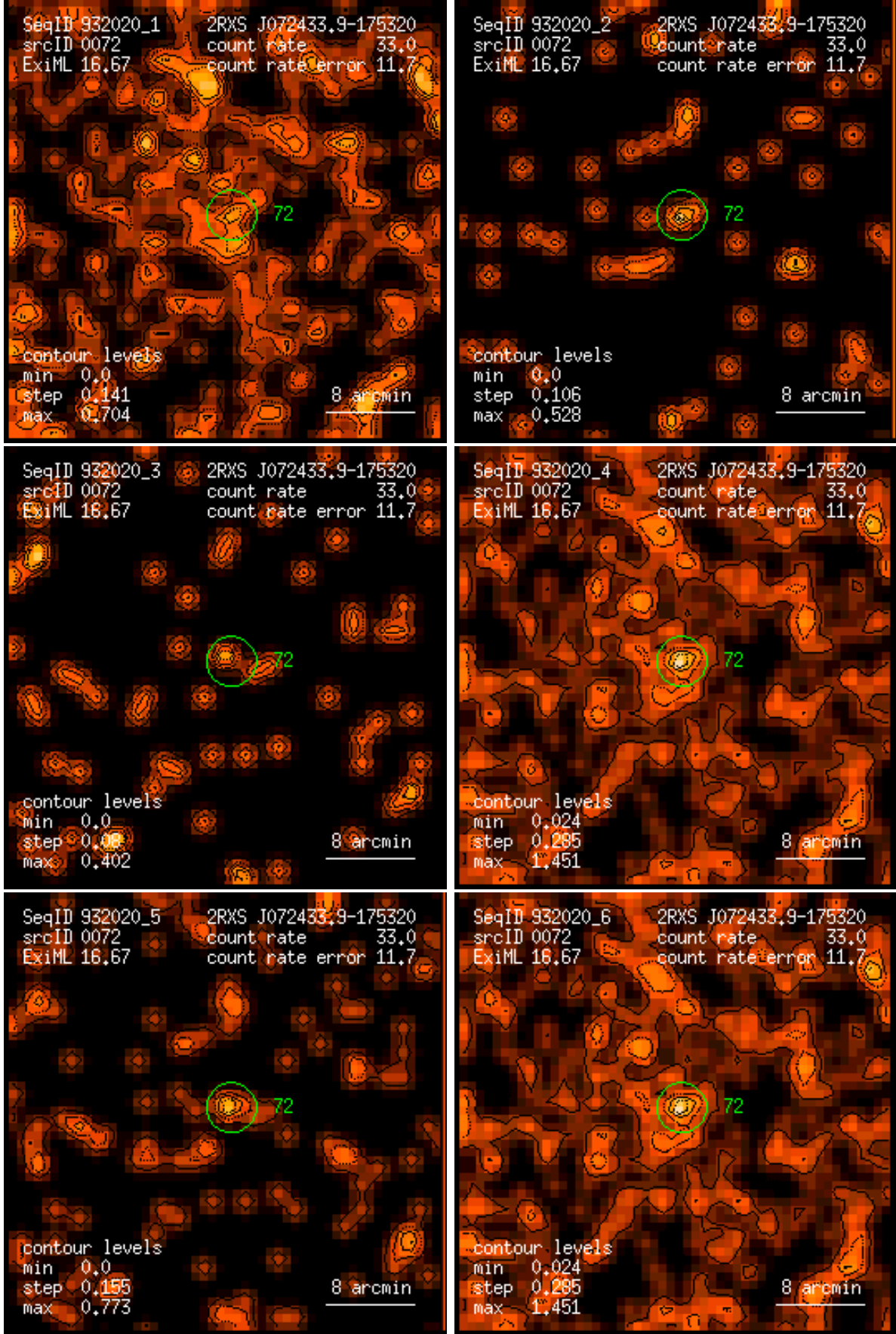
Figure 72: RASS 932020: detection 0072: band rate images, Gaussian filter: (1) PSPC channels 11 – 41, (2) 52 – 90, (3) 91 – 201, (4) 11 – 235, (5) 52 – 201, (6) 11 – 201. Broad band rates in counts/ks. Band rate contour levels in counts/ks/arcmin 2 .
