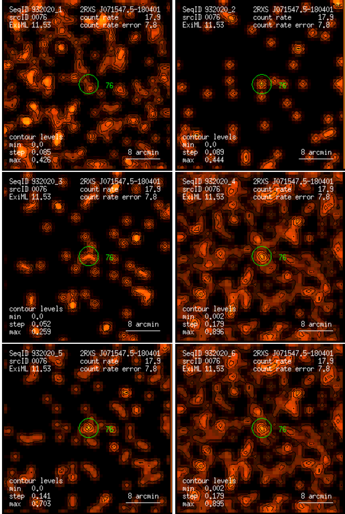
Figure 76: RASS 932020: detection 0076: band rate images, Gaussian filter: (1) PSPC channels 11 – 41, (2) 52 – 90, (3) 91 – 201, (4) 11 – 235, (5) 52 – 201, (6) 11 – 201. Broad band rates in counts/ks. Band rate contour levels in counts/ks/arcmin 2 .
