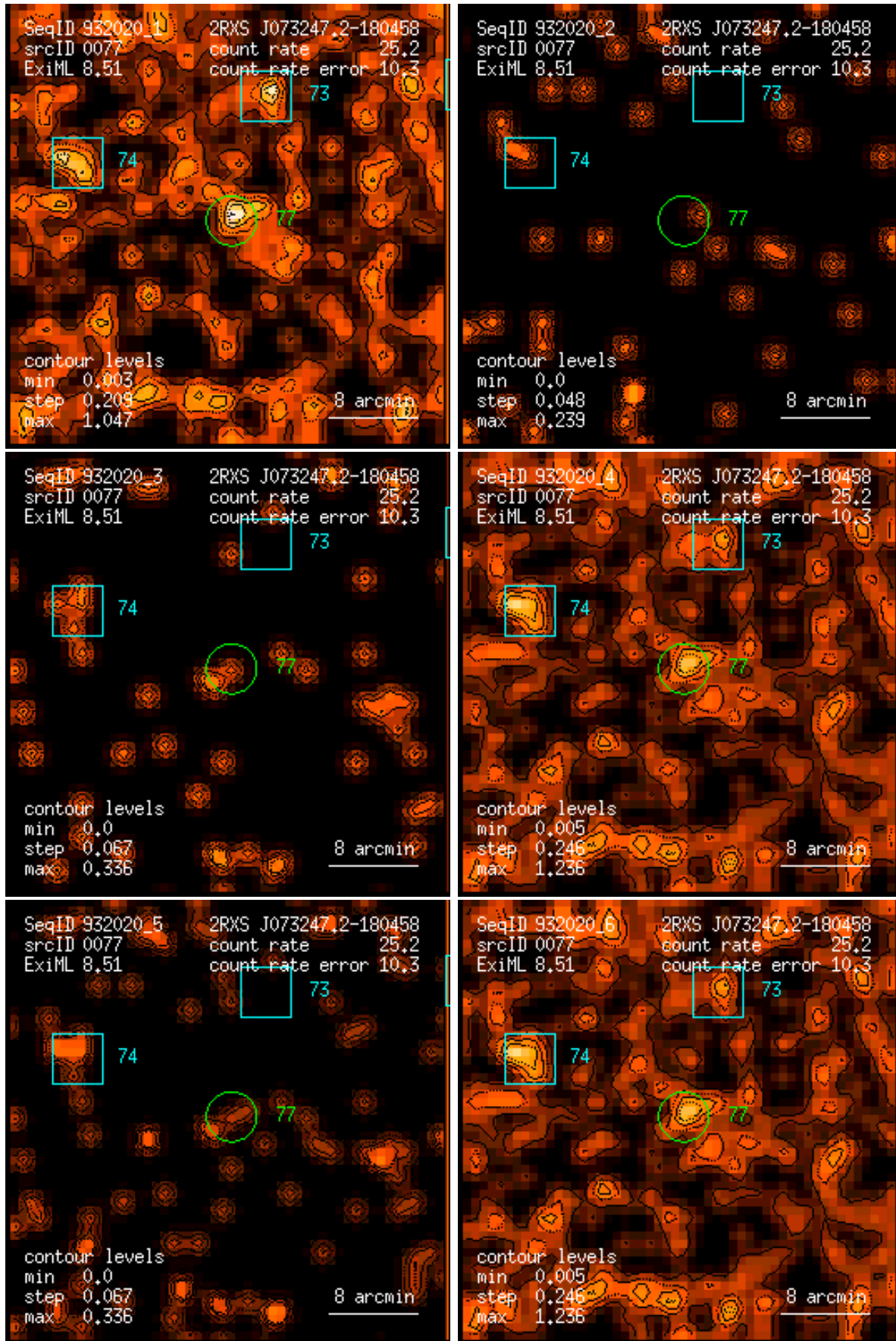
Figure 77: RASS 932020: detection 0077: band rate images, Gaussian filter: (1) PSPC channels 11 – 41, (2) 52 – 90, (3) 91 – 201, (4) 11 – 235, (5) 52 – 201, (6) 11 – 201. Broad band rates in counts/ks. Band rate contour levels in counts/ks/arcmin 2 .
