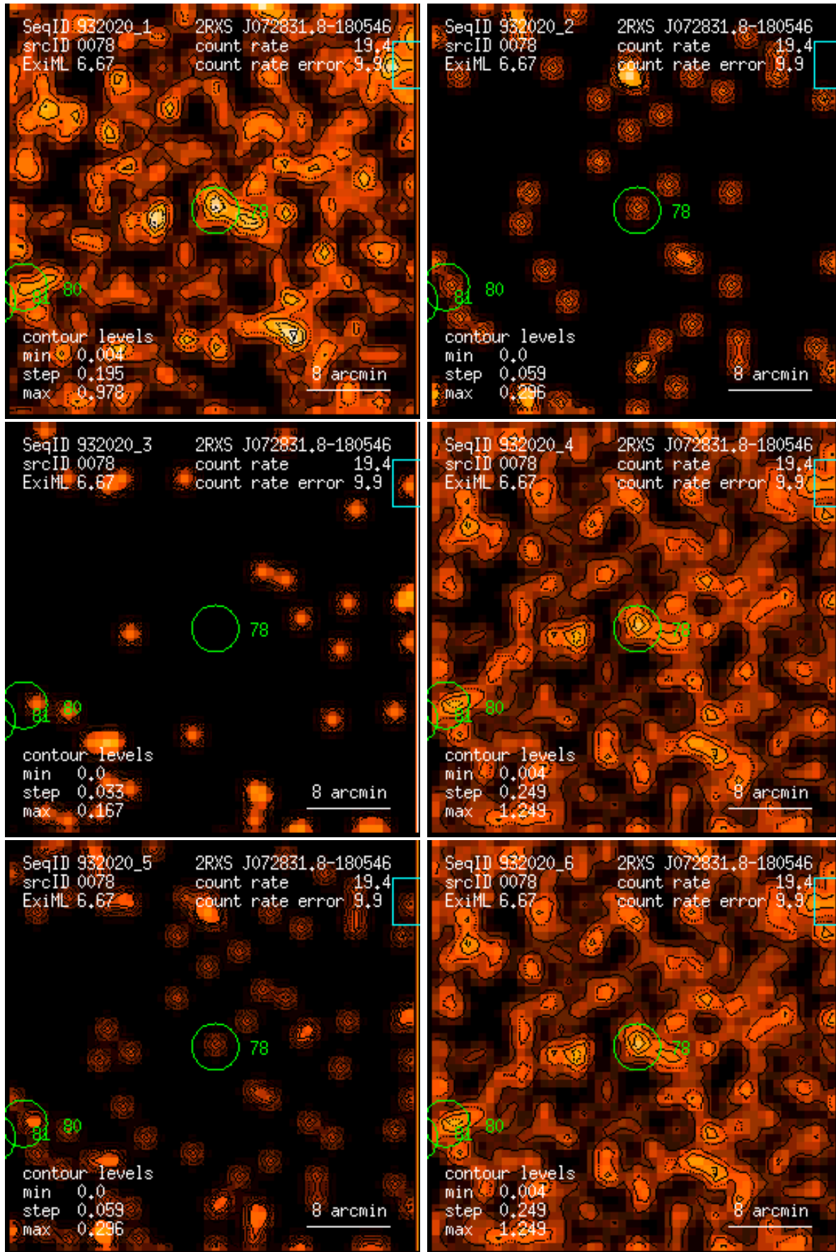
Figure 78: RASS 932020: detection 0078: band rate images, Gaussian filter: (1) PSPC channels 11 – 41, (2) 52 – 90, (3) 91 – 201, (4) 11 – 235, (5) 52 – 201, (6) 11 – 201. Broad band rates in counts/ks. Band rate contour levels in counts/ks/arcmin 2 .
