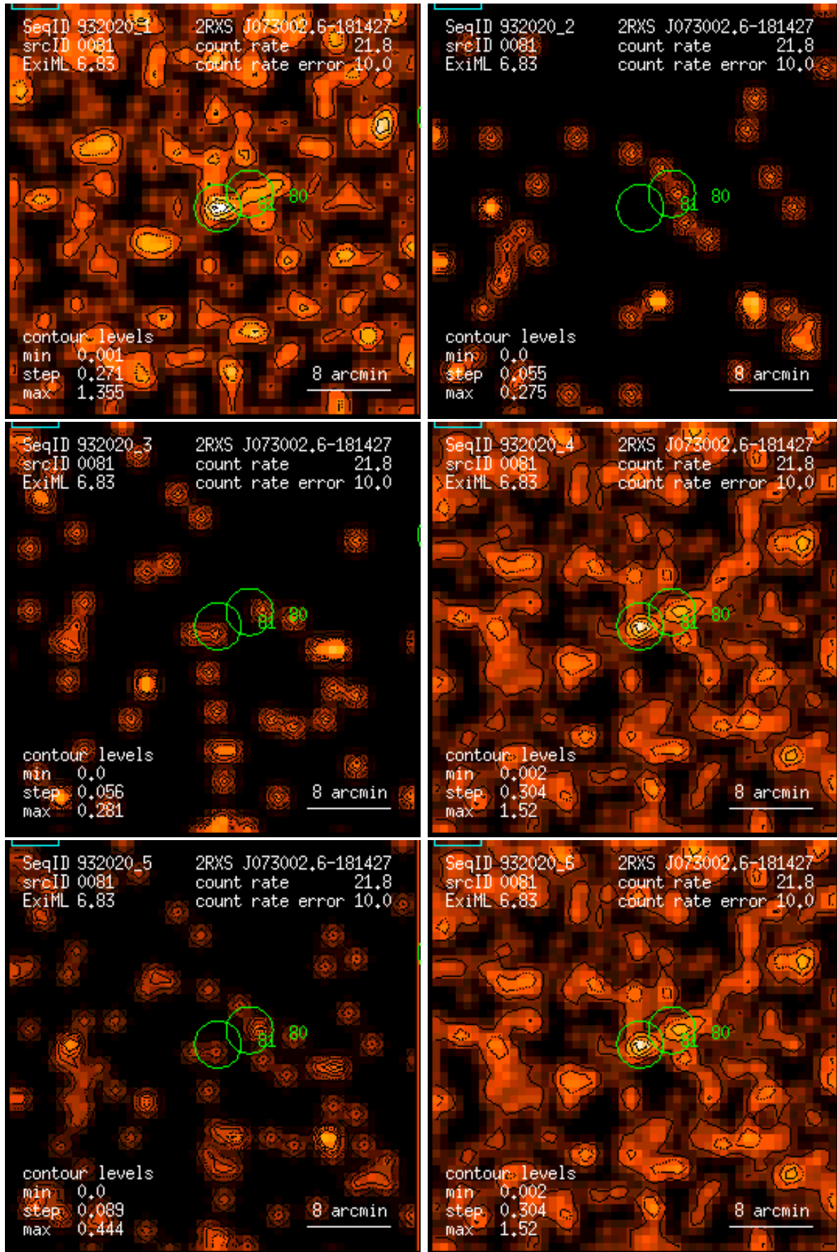
Figure 81: RASS 932020: detection 0081: band rate images, Gaussian filter: (1) PSPC channels 11 – 41, (2) 52 – 90, (3) 91 – 201, (4) 11 – 235, (5) 52 – 201, (6) 11 – 201. Broad band rates in counts/ks. Band rate contour levels in counts/ks/arcmin 2 .
