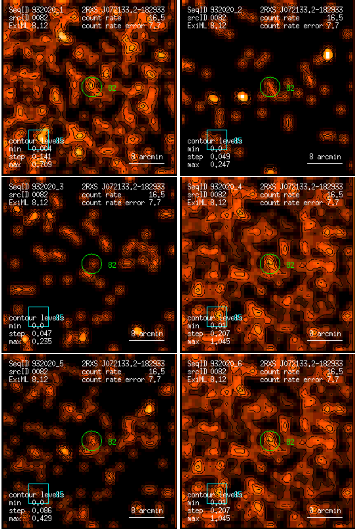
Figure 82: RASS 932020: detection 0082: band rate images, Gaussian filter: (1) PSPC channels 11 – 41, (2) 52 – 90, (3) 91 – 201, (4) 11 – 235, (5) 52 – 201, (6) 11 – 201. Broad band rates in counts/ks. Band rate contour levels in counts/ks/arcmin 2 .
