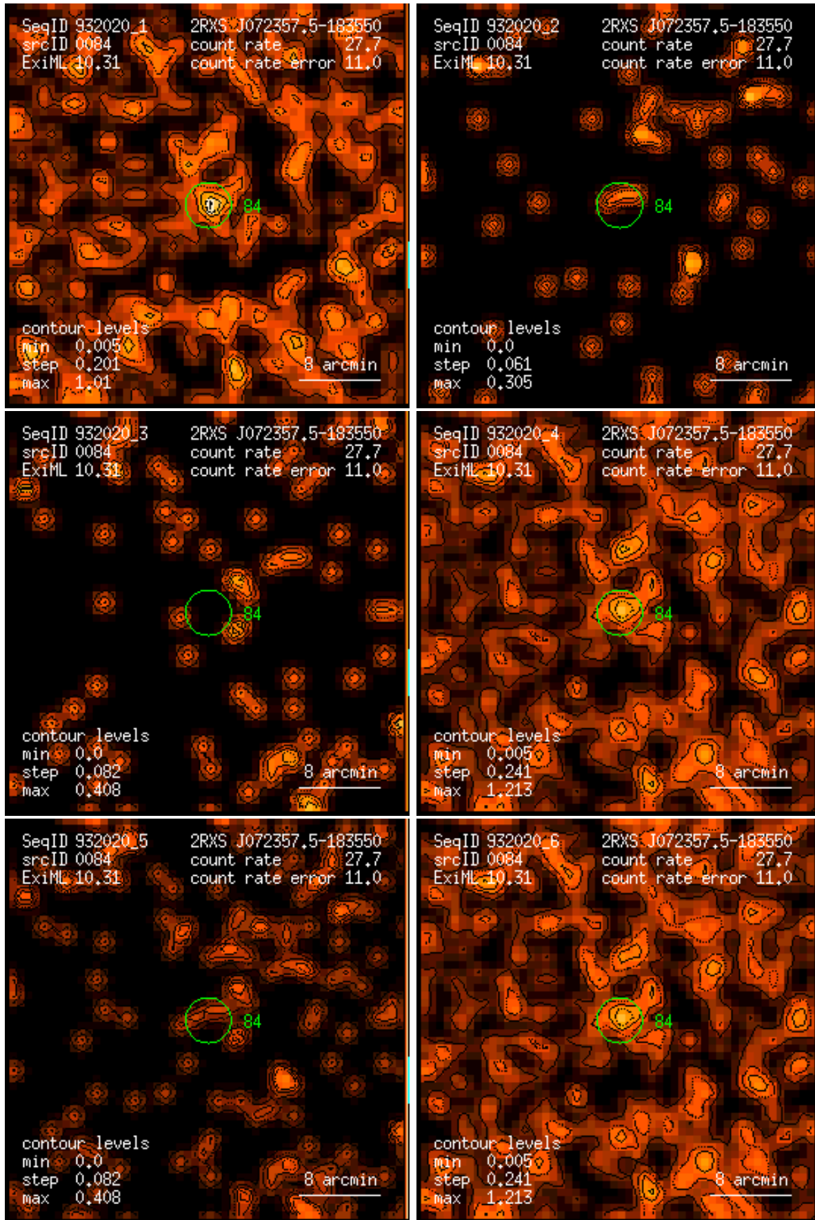
Figure 84: RASS 932020: detection 0084: band rate images, Gaussian filter: (1) PSPC channels 11 – 41, (2) 52 – 90, (3) 91 – 201, (4) 11 – 235, (5) 52 – 201, (6) 11 – 201. Broad band rates in counts/ks. Band rate contour levels in counts/ks/arcmin 2 .
