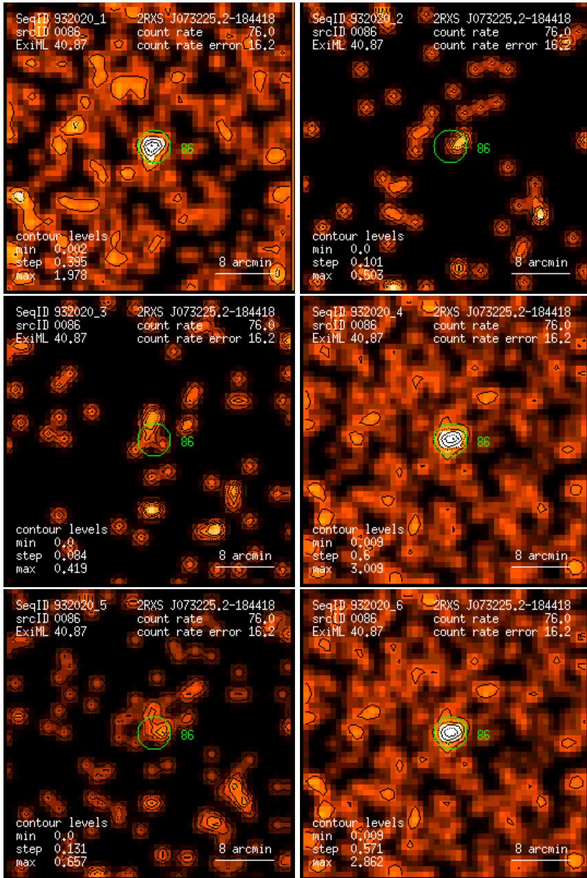
Figure 86: RASS 932020: detection 0086: band rate images, Gaussian filter: (1) PSPC channels 11 – 41, (2) 52 – 90, (3) 91 – 201, (4) 11 – 235, (5) 52 – 201, (6) 11 – 201. Broad band rates in counts/ks. Band rate contour levels in counts/ks/arcmin 2 .
