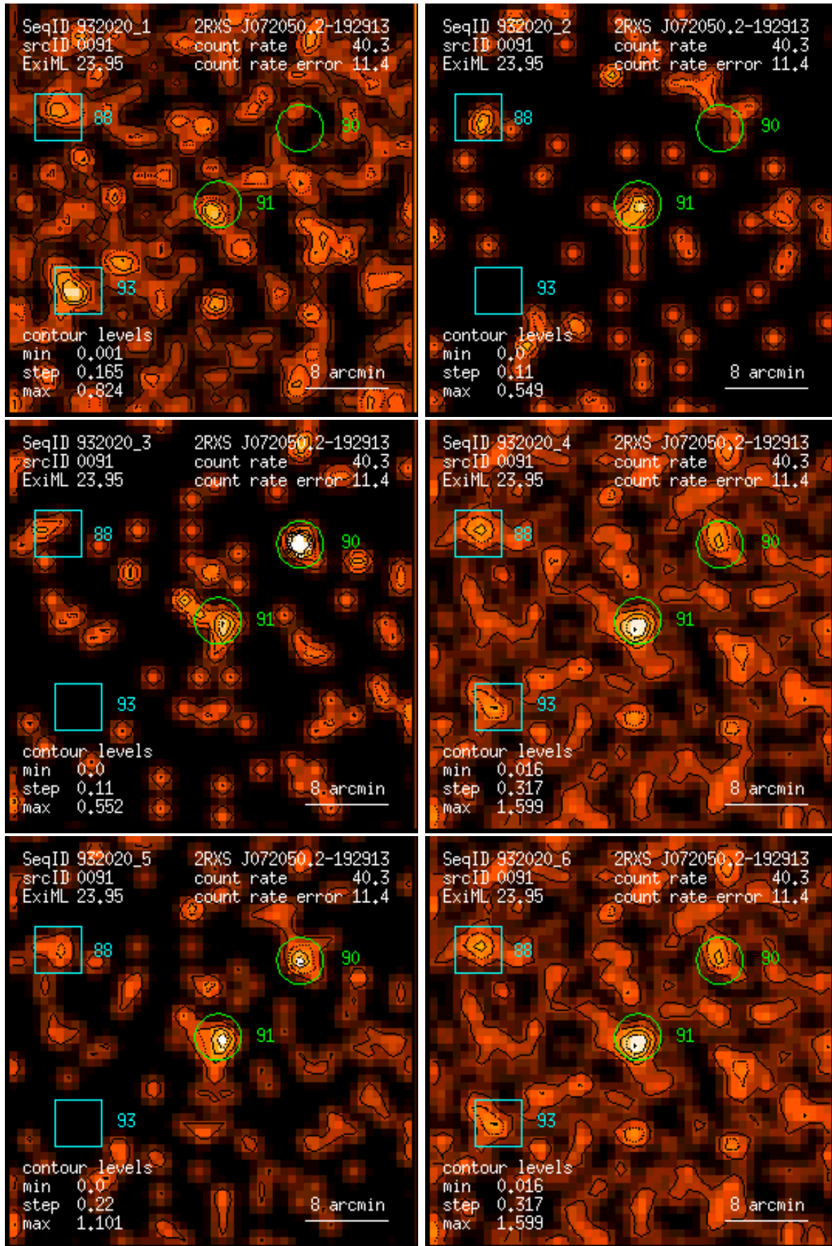
Figure 91: RASS 932020: detection 0091: band rate images, Gaussian filter: (1) PSPC channels 11 – 41, (2) 52 – 90, (3) 91 – 201, (4) 11 – 235, (5) 52 – 201, (6) 11 – 201. Broad band rates in counts/ks. Band rate contour levels in counts/ks/arcmin 2 .
