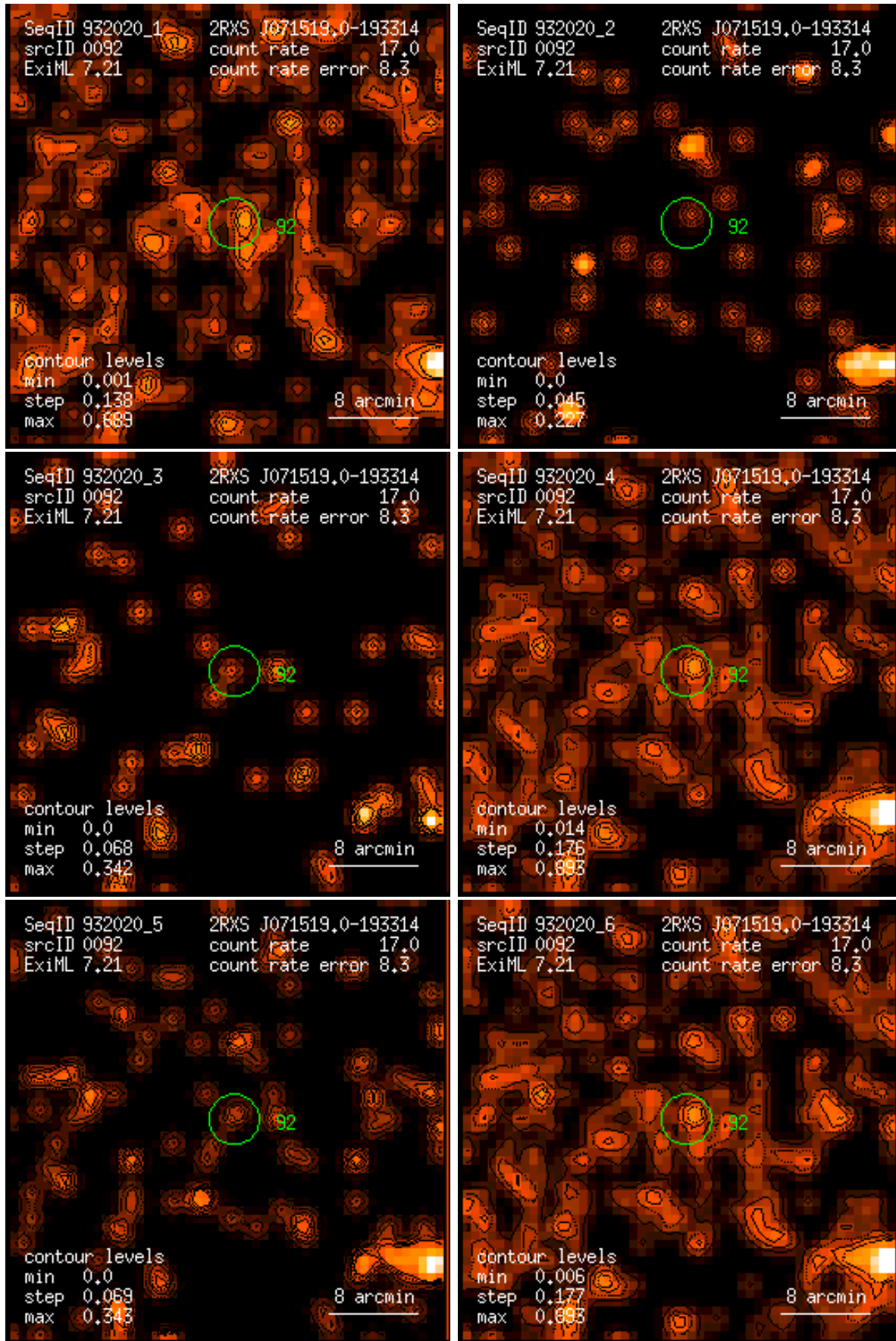
Figure 92: RASS 932020: detection 0092: band rate images, Gaussian filter: (1) PSPC channels 11 – 41, (2) 52 – 90, (3) 91 – 201, (4) 11 – 235, (5) 52 – 201, (6) 11 – 201. Broad band rates in counts/ks. Band rate contour levels in counts/ks/arcmin 2 .
