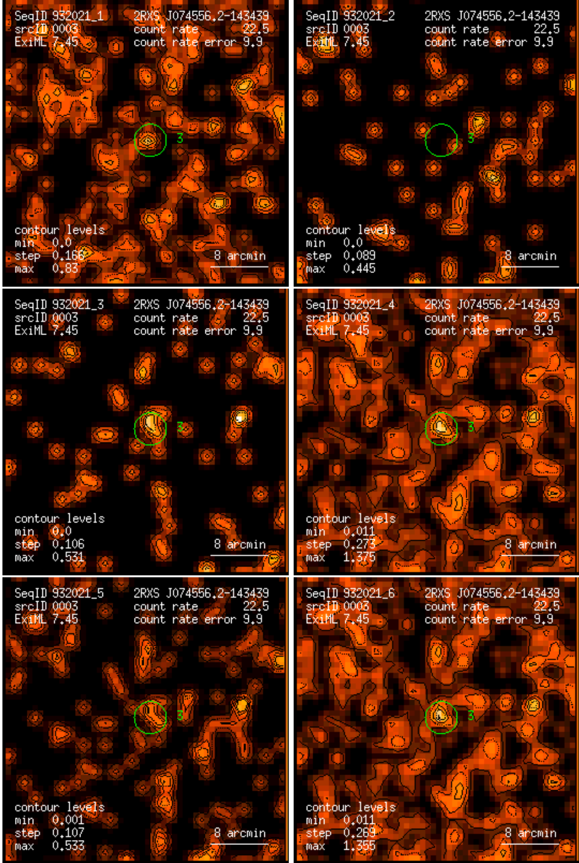
Figure 3: RASS 932021: detection 0003: band rate images, Gaussian filter: (1) PSPC channels 11 – 41, (2) 52 – 90, (3) 91 – 201, (4) 11 – 235, (5) 52 – 201, (6) 11 – 201. Broad band rates in counts/ks. Band rate contour levels in counts/ks/arcmin 2 .
