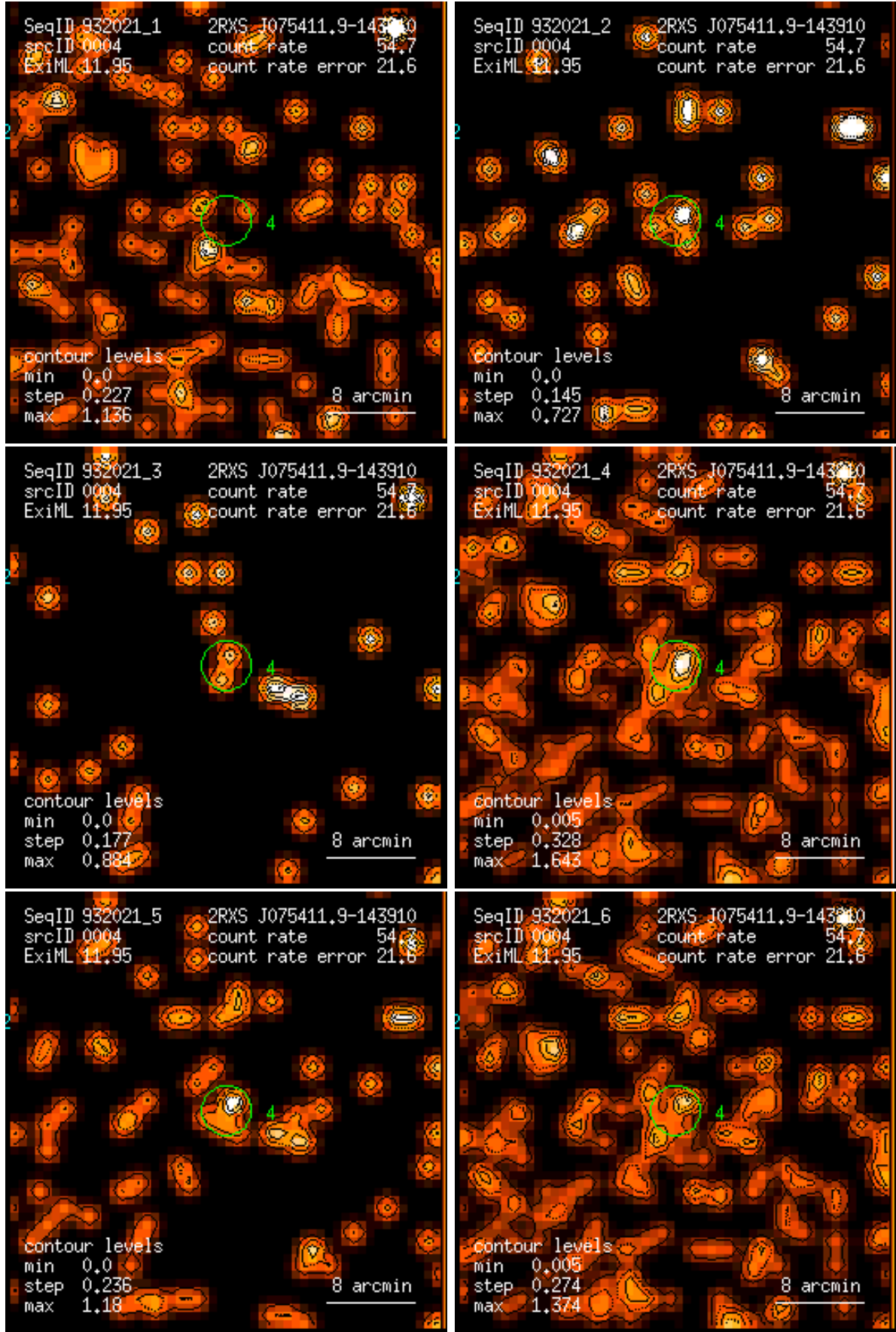
Figure 4: RASS 932021: detection 0004: band rate images, Gaussian filter: (1) PSPC channels 11 – 41, (2) 52 – 90, (3) 91 – 201, (4) 11 – 235, (5) 52 – 201, (6) 11 – 201. Broad band rates in counts/ks. Band rate contour levels in counts/ks/arcmin 2 .
