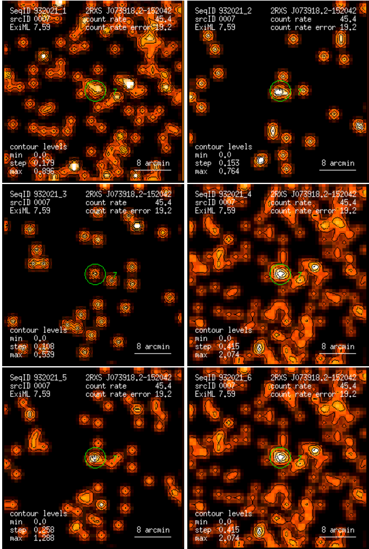
Figure 7: RASS 932021: detection 0007: band rate images, Gaussian filter: (1) PSPC channels 11 – 41, (2) 52 – 90, (3) 91 – 201, (4) 11 – 235, (5) 52 – 201, (6) 11 – 201. Broad band rates in counts/ks. Band rate contour levels in counts/ks/arcmin 2 .
