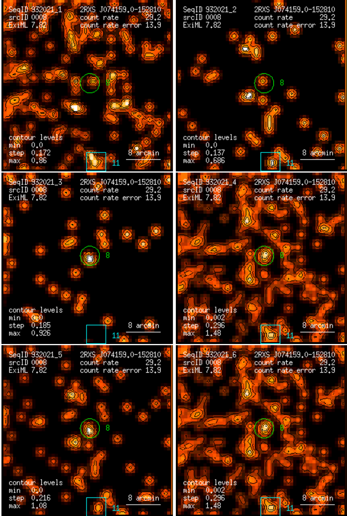
Figure 8: RASS 932021: detection 0008: band rate images, Gaussian filter: (1) PSPC channels 11 – 41, (2) 52 – 90, (3) 91 – 201, (4) 11 – 235, (5) 52 – 201, (6) 11 – 201. Broad band rates in counts/ks. Band rate contour levels in counts/ks/arcmin 2 .
