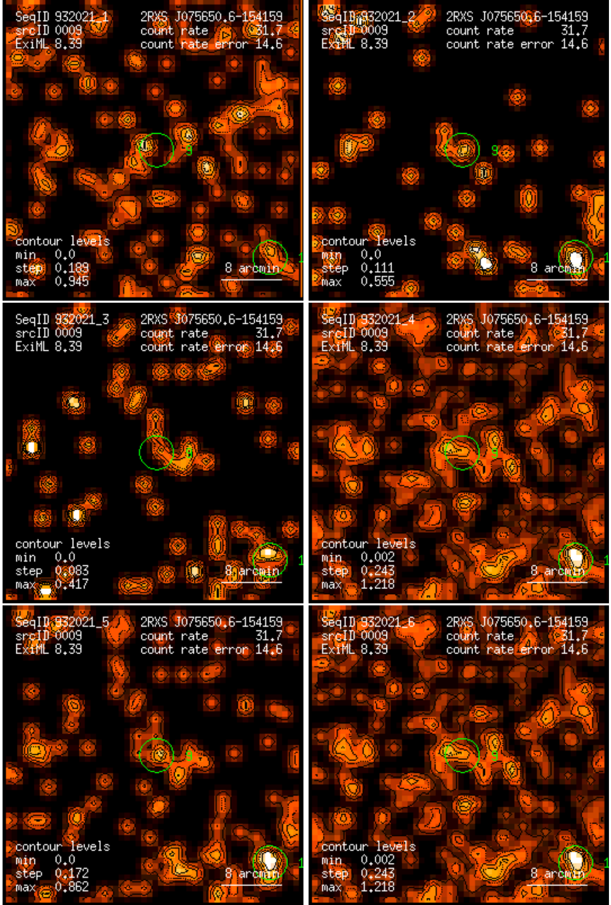
Figure 9: RASS 932021: detection 0009: band rate images, Gaussian filter: (1) PSPC channels 11 – 41, (2) 52 – 90, (3) 91 – 201, (4) 11 – 235, (5) 52 – 201, (6) 11 – 201. Broad band rates in counts/ks. Band rate contour levels in counts/ks/arcmin 2 .
