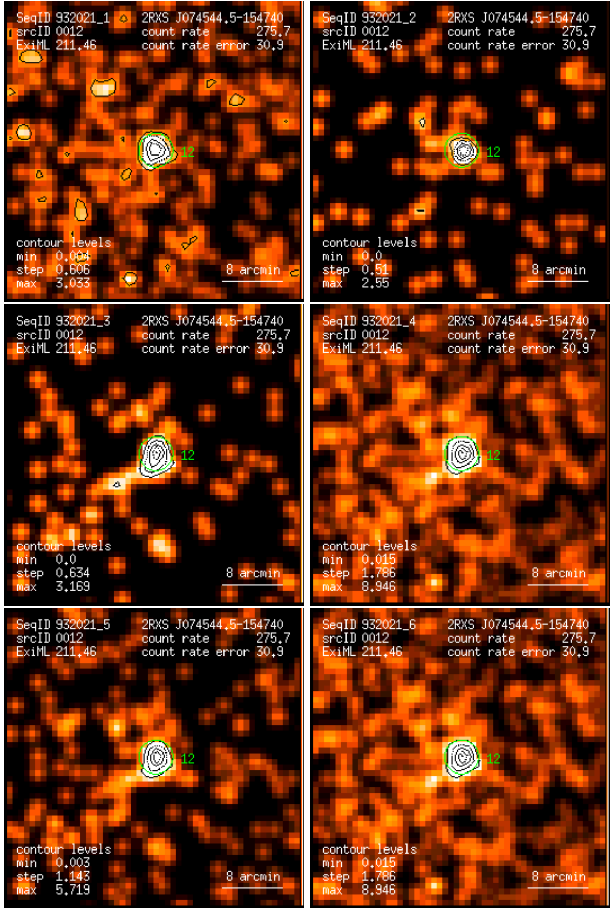
Figure 12: RASS 932021: detection 0012: band rate images, Gaussian filter: (1) PSPC channels 11 – 41, (2) 52 – 90, (3) 91 – 201, (4) 11 – 235, (5) 52 – 201, (6) 11 – 201. Broad band rates in counts/ks. Band rate contour levels in counts/ks/arcmin 2 .
