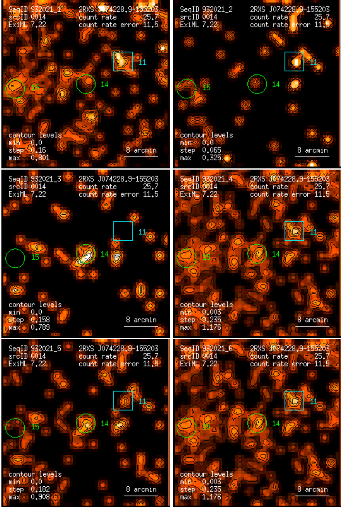
Figure 14: RASS 932021: detection 0014: band rate images, Gaussian filter: (1) PSPC channels 11 – 41, (2) 52 – 90, (3) 91 – 201, (4) 11 – 235, (5) 52 – 201, (6) 11 – 201. Broad band rates in counts/ks. Band rate contour levels in counts/ks/arcmin 2 .
