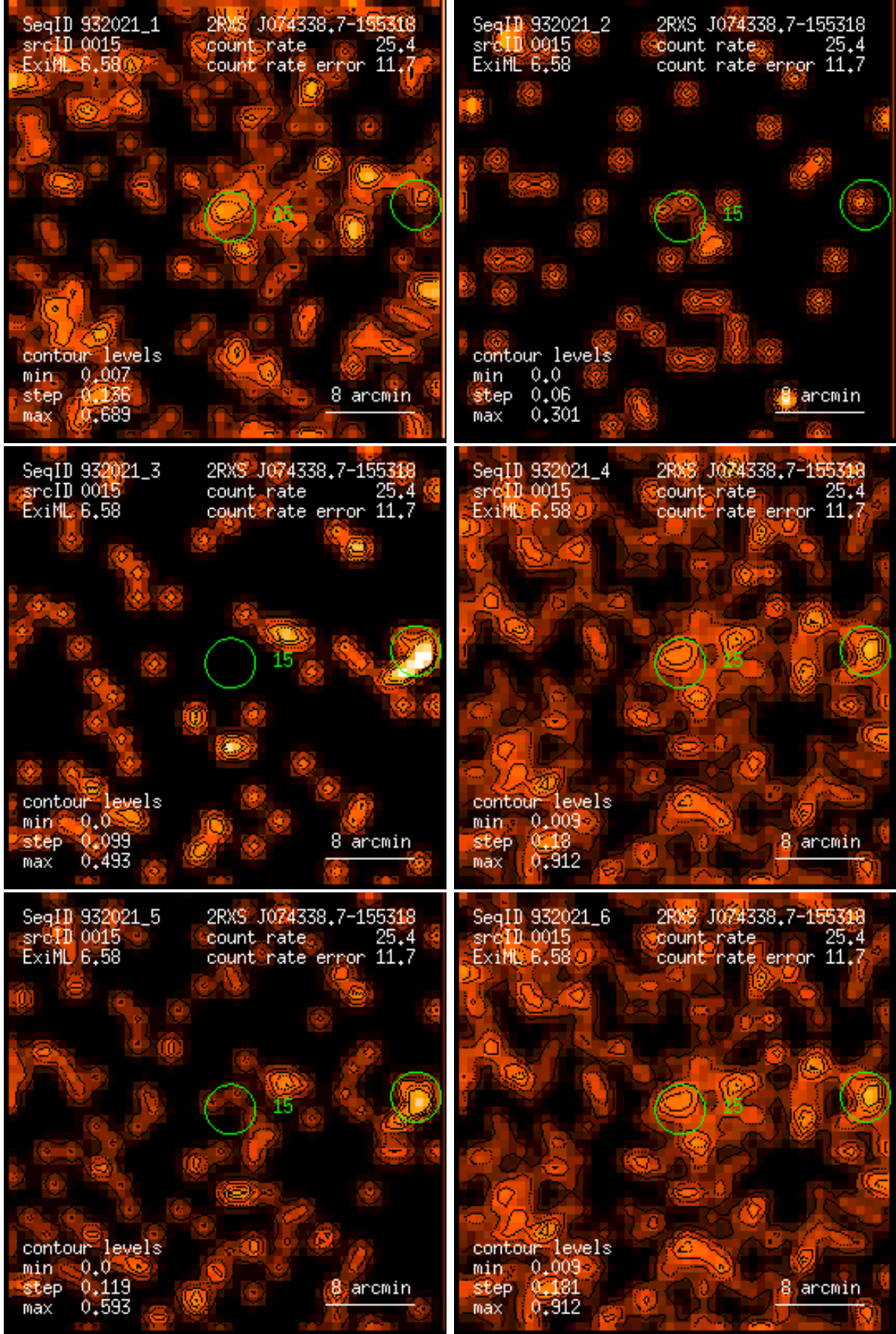
Figure 15: RASS 932021: detection 0015: band rate images, Gaussian filter: (1) PSPC channels 11 – 41, (2) 52 – 90, (3) 91 – 201, (4) 11 – 235, (5) 52 – 201, (6) 11 – 201. Broad band rates in counts/ks. Band rate contour levels in counts/ks/arcmin 2 .
