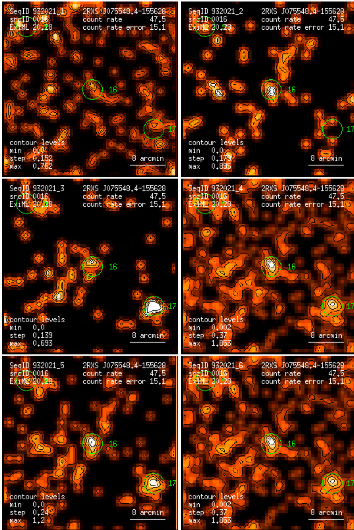
Figure 16: RASS 932021: detection 0016: band rate images, Gaussian filter: (1) PSPC channels 11 – 41, (2) 52 – 90, (3) 91 – 201, (4) 11 – 235, (5) 52 – 201, (6) 11 – 201. Broad band rates in counts/ks. Band rate contour levels in counts/ks/arcmin 2 .
